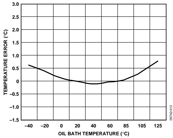
Figure 11. Internal Temperature Error vs. ADT7476A Temperature
