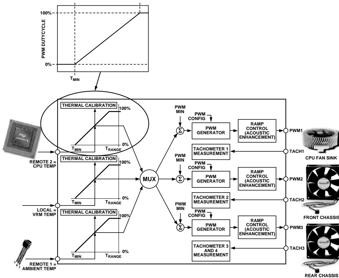
Figure 53. Understanding the T_{MIN} Parameter
