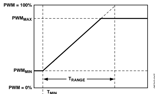
Figure 46. T_{RANGE}
