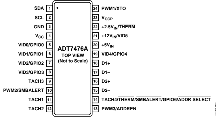
Figure 3. Pin Configuration
