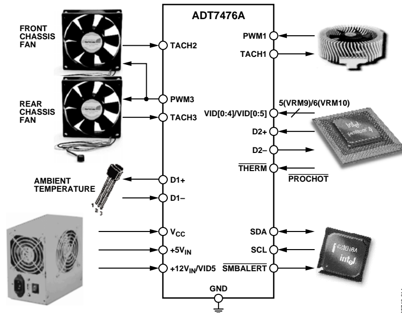
Figure 13. ADT7476A Configuration
