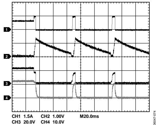
Figure 47. Overcurrent Condition During Operation (ADM1177-2 Model) (CH1 = I_{LOAD} , CH2 = V_{TIMER} , CH3 = V_{GATE} , CH4 = V_{OUT} )
