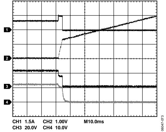
Figure 46. Overcurrent Condition During Operation (ADM1177-1 Model) (CH1 = I_{LOAD} , CH2 = V_{TIMER} , CH3 = V_{GATE} , CH4 = V_{OUT} )
