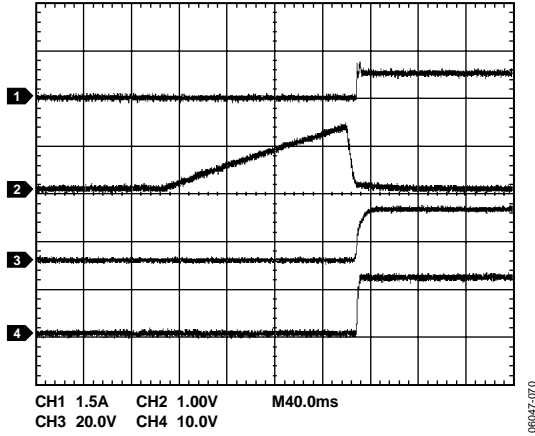
Figure 43. Inrush Current Control into 220 \mu F Load (CH1 = I_{LOAD} , CH2 = V_{TIMER} , CH3 = V_{GATE} , CH4 = V_{OUT} )
