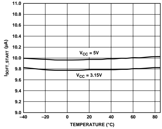
Figure 30. SS Pin Pull-Up Current vs. Temperature
