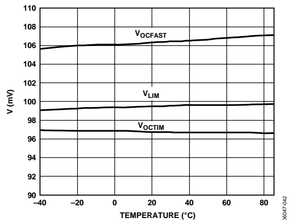
Figure 23. V OCTIM , V LIM , V OFAST vs. Temperature
