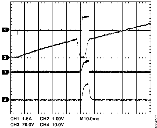
Figure 44. Overcurrent Condition at Startup (ADM1177-1 Model) (CH1 = I_{LOAD} , CH2 = V_{TIMER} , CH3 = V_{GATE} , CH4 = V_{OUT} )
