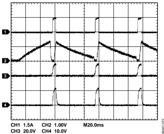
Figure 45. Overcurrent Condition at Startup (ADM1177-2 Model) (CH1 = I_{LOAD} , CH2 = V_{TIMER} , CH3 = V_{GATE} , CH4 = V_{OUT} )
