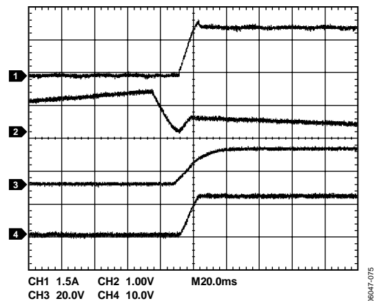
Figure 48. Inrush Current Control with Profiling of Initial Current Edge via a Capacitor on the SS Pin (CH1 = I_{LOAD} , CH2 = V_{TIMER} , CH3 = V_{GATE} , CH4 = V_{OUT} )
