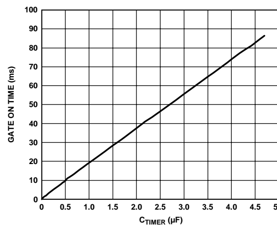
Figure 15. Current Limit On Time vs. Timer Capacitance
