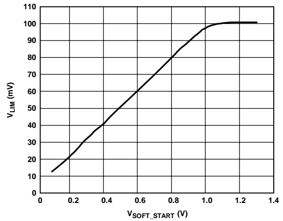
Figure 31. V_{LIM} vs. V_{SS}
