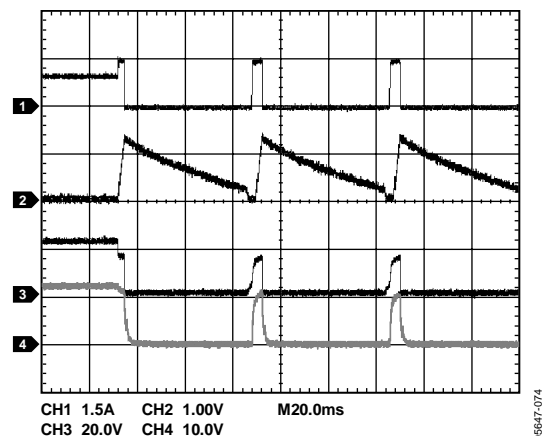
Figure 45. Overcurrent Condition During Operation (ADM1175-2 Model) (CH1 = I_{LOAD} , CH2 = V_{TIMER} , CH3 = V_{GATE} , CH4 = V_{OUT} )
