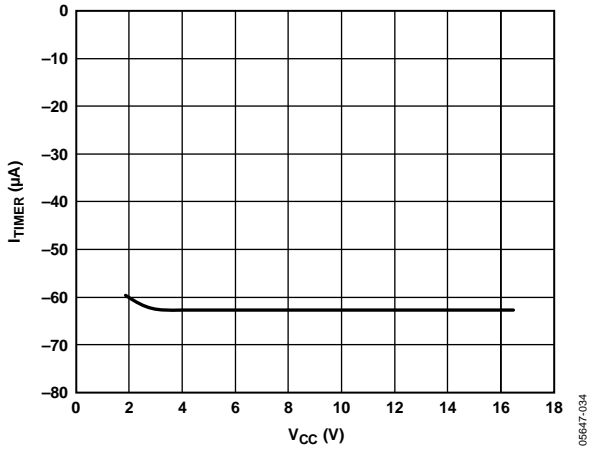
Figure 17. Timer Pull-Up Current (C. B. Delay) vs. Supply Voltage
