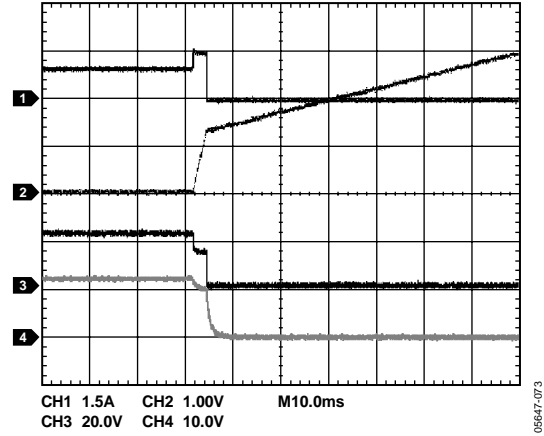
Figure 44. Overcurrent Condition During Operation (ADM1175-1 Model) (CH1 = I_{LOAD} , CH2 = V_{TIMER} , CH3 = V_{GATE} , CH4 = V_{OUT} )
