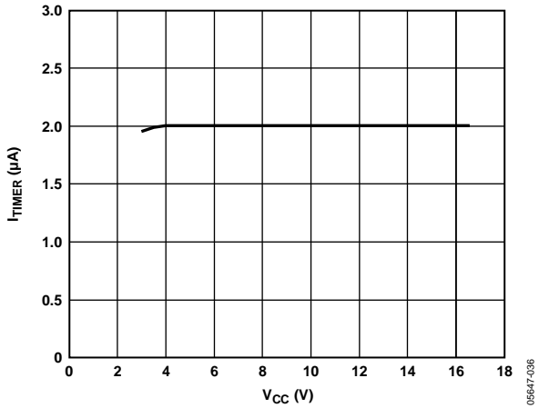
Figure 18. Timer Pull-Down Current (Cool-Off Cycle) vs. Supply Voltage
