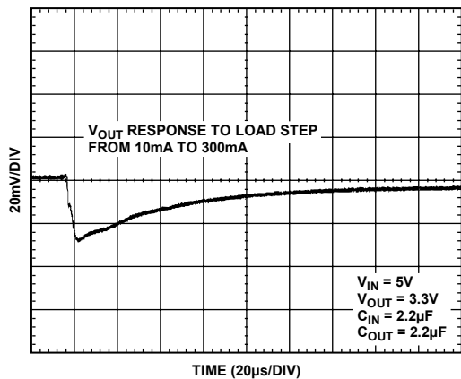
Figure 31. Output Transient Response, C_{\text{OUT}} = 2.2 \mu\text{F}
