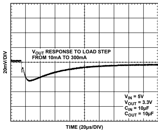
Figure 32. Output Transient Response, C_{\text{OUT}} = 10 \mu\text{F}
