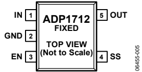
Figure 5. 5-Lead TSOT (UJ-Suffix)
