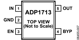
Figure 7. 5-Lead TSOT (UJ-Suffix)
