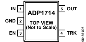
Figure 8. 5-Lead TSOT (UJ-Suffix)
