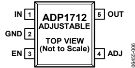
Figure 6. 5-Lead TSOT (UJ-Suffix)
