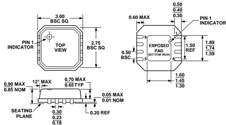
Figure 19. 8-Lead Lead Frame Chip Scale Package [LFCSP_VD] 3 mm x 3 mm Body, Very Thin, Dual Lead (CP-8-2) Dimensions shown in millimeters
