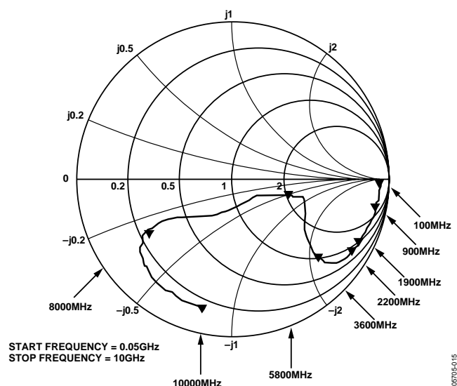
Figure 15. Input Impedance vs. Frequency; No Termination Resistor on INH1 (Impedance De-Embedded to Input Pins), Z_0 = 50 \Omega
