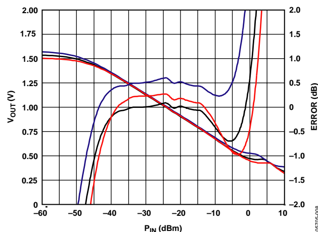
Figure 8. V_{OUT} and Log Conformance vs. Input Amplitude at 8.0 GHz, R_{TADJ} = \text{Open} , Error Calculated from P_{IN} = -34\text{ dBm} to P_{IN} = -16\text{ dBm}
