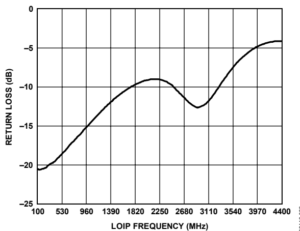
Figure 23. LO Port Input Return Loss vs. Frequency
