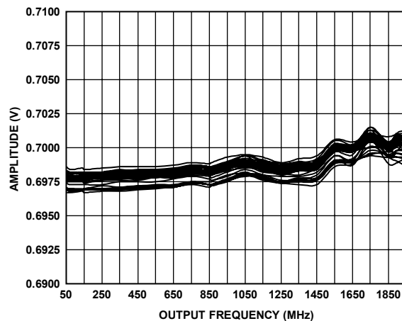
Figure 12. Distribution of Peak Q Amplitude to Null Undesired Sideband (Peak I Amplitude Held Constant at 0.7 V)
