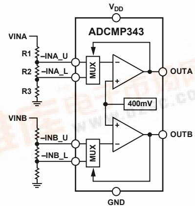
Figure 2. ADCMP343
