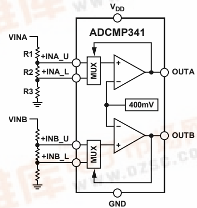
Figure 1. ADCMP341
