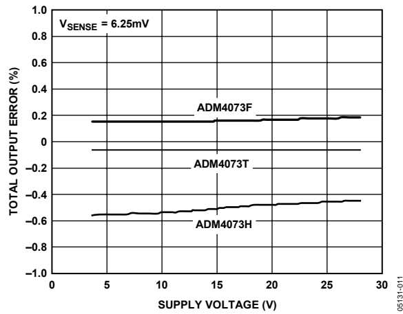
Figure 10. Total Output Error vs. Supply Voltage ( V_{SENSE} = 6.25mV )
