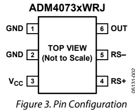
Figure 3. Pin Configuration
