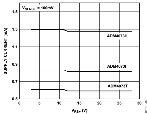
Figure 8. Supply Current vs. RS+ Voltage ( V_{SENSE} = 100mV )
