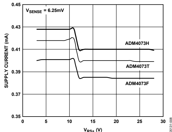
Figure 7. Supply Current vs. RS+ Voltage ( V_{SENSE} = 6.25mV )
