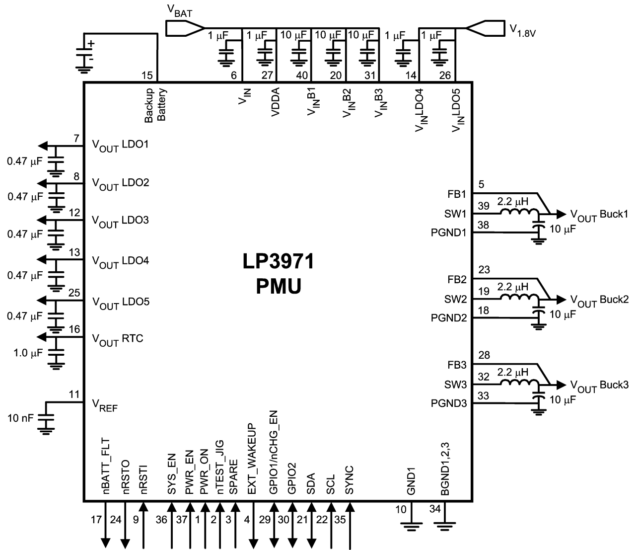
Diagram 2 LDO 4 and LDO5 Connected To 1.8V Supply
