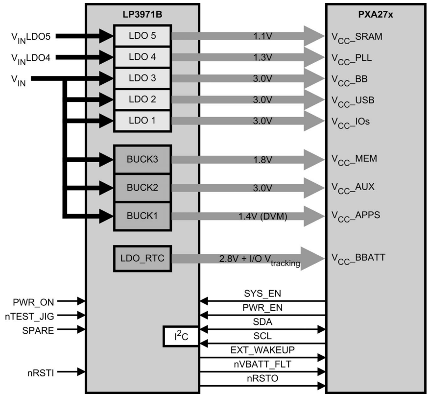
Typical Application Diagram with PXA27x Advanced Applications Processor Version "B"
