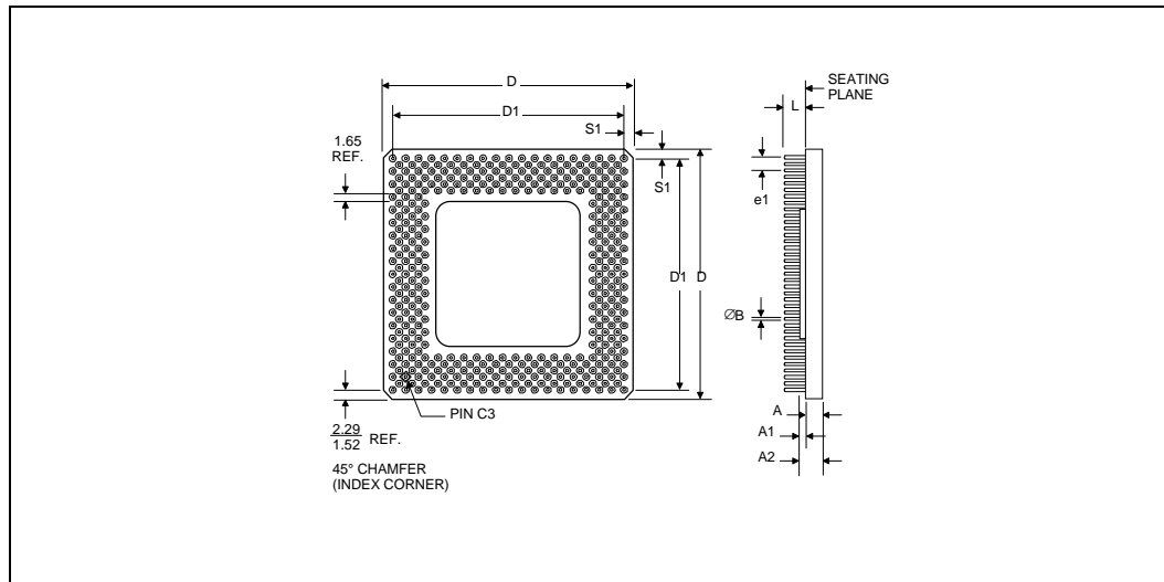
Figure 13. SPGA Package Dimensions without Heat Spreader
