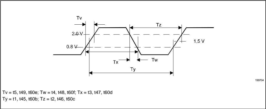
Figure 4. Clock Waveform
