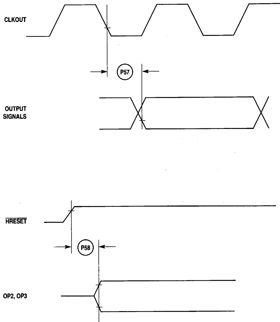
Figure 20-26. PCMCIA Output Port Timing Diagram
