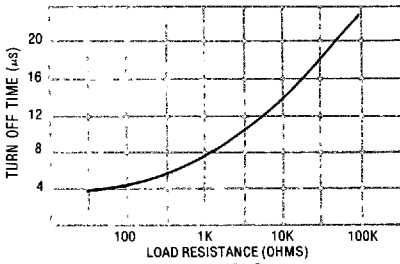
FIGURE 7 - TURN OFF TIME VS. LOAD RESISTANCE (TYPICAL)
