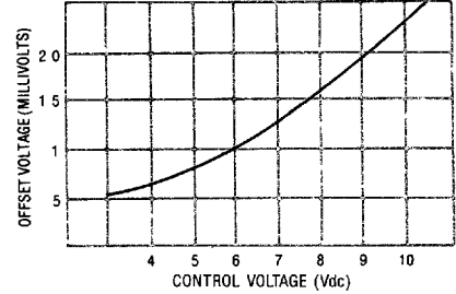
FIGURE 3 - OFFSET VOLTAGE VS. INPUT CONTROL VOLTAGE (TYPICAL)
