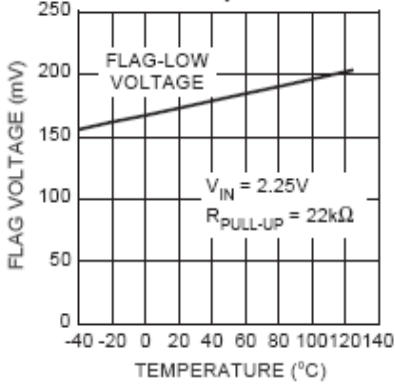
Flag-Low Voltage vs. Temperature
