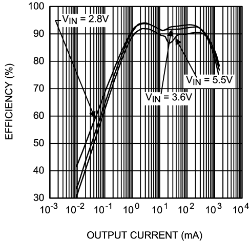
Buck 1 Efficiency vs Output Current (PFM to PWM mode, V_{out} = 1.2\text{V} , L = 2.2\mu\text{H} )
