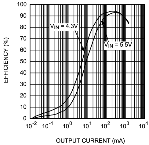
Buck 2 Efficiency vs Output Current (Forced PWM Mode, V_{out} = 1.8\text{V} , L = 2.2\mu\text{H} )
