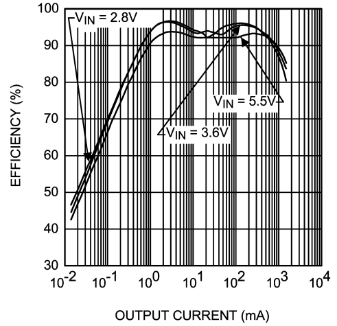
Buck 1 Efficiency vs Output Current (PFM to PWM mode, V_{out} = 2.0\text{V} , L = 2.2\mu\text{H} )
