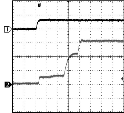
Start up into PWM Mode Vout = 3.3 V, 1.2 A load
