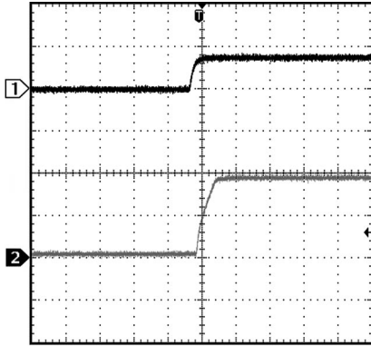
Start up into PFM Mode Vout = 1.8 V, 30 mA load
