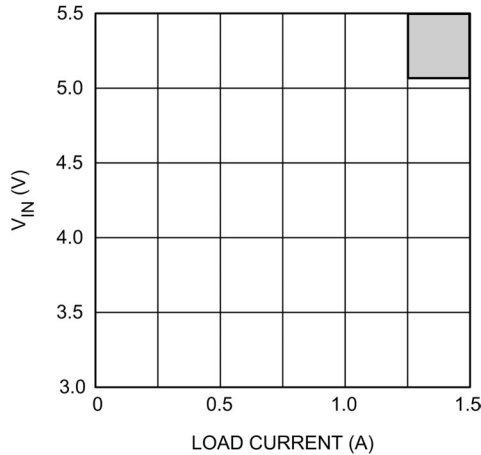
LP3906 Buck Converter VIN vs ILOAD Operating Ranges
