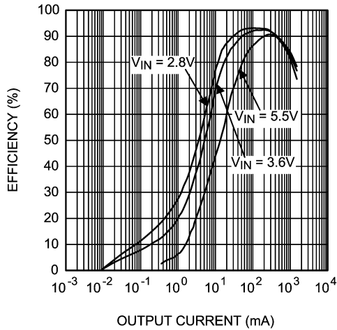
Buck 1 Efficiency vs Output Current (Forced PWM Mode, Vout = 1.2V, L = 2.2µH)
