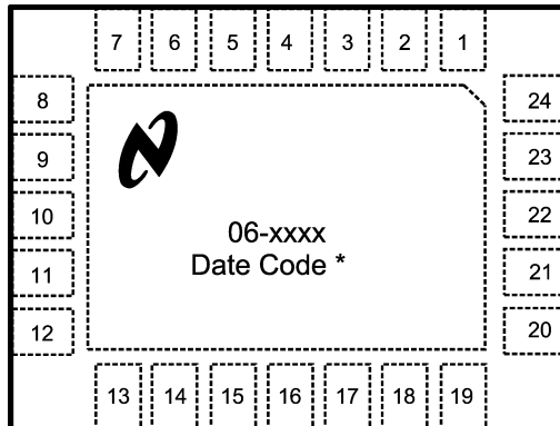
FIGURE 3. 24-Lead LLP Package (Top View)
