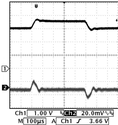
Line Transient Response V_{in} = 3 - 3.6\text{V} , V_{out} = 1.2\text{V} , 250 mA load
