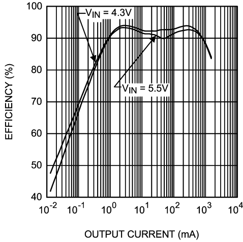
Buck 2 Efficiency vs Output Current (PFM to PWM Mode, V_{out} = 1.8\text{V} , L = 2.2\mu\text{H} )
