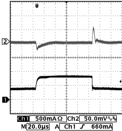
Load Transient Response V_{out} = 1.2\text{V} (PWM Mode)
