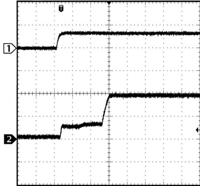
Start up into PWM Mode Vout = 1.8 V, 1.2 A load
