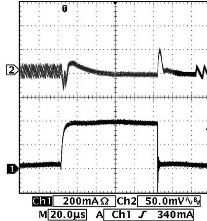
Mode Change by Load Transient V_{out} = 1.2\text{V} (PWM to PFM)
