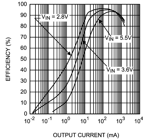
Buck 1 Efficiency vs Output Current (Forced PWM Mode, Vout = 2.0V, L = 2.2µH)
