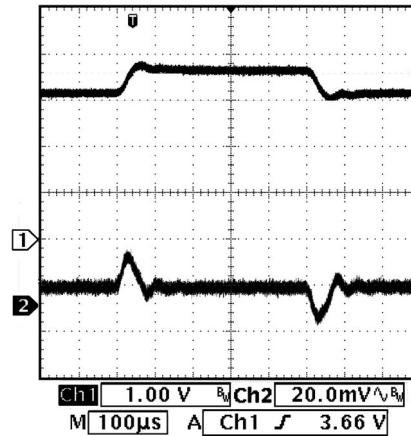
Line Transient Response V_{in} = 3 - 3.6\text{V} , V_{out} = 3.3\text{V} , 250 mA load
