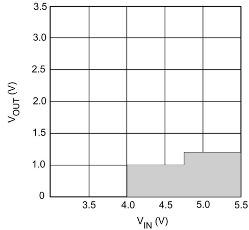
LP3906 Buck Converter V_{OUT} vs V_{IN} Operating Range during PFM-PWM-PPM Transition
