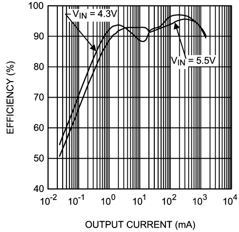
Buck 2 Efficiency vs Output Current (PFM to PWM Mode, V_{out} = 3.3\text{V} , L = 2.2\mu\text{H} )
