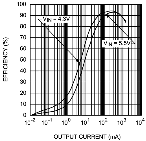
Buck 2 Efficiency vs Output Current (Forced PWM Mode, V_{out} = 3.3\text{V} , L = 2.2\mu\text{H} )
