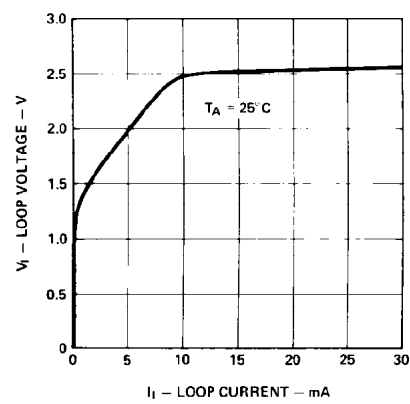
Figure 4. Typical Input Loop Voltage vs. Input Current.
