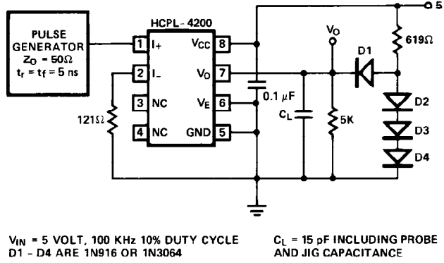
Figure 8. Test Circuit for t_{PHL} , t_{PLH} , t_r , and t_f .
