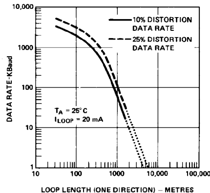
Figure 20. Typical Data Rate vs. Loop Length (One Direction) - Distance.
