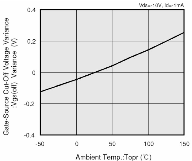
Fig 6. Gate-Source Cut-off Voltage Variance vs. Ambient Temperature
