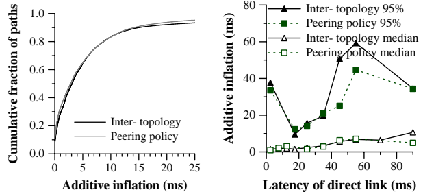
Figure 15: Path inflation due to inter-domain topology relative to a hypothetical direct link. Each ISP chooses a lowest-latency path to reach destinations. The peering policy line represents the inflation caused by the factors in Sections 4 and 5.
