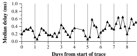
Figure 11: The median delay on the San Francisco peering between AT&T and Sprint with 4 hour averaging. The vertical bars represent midnight on each day.
