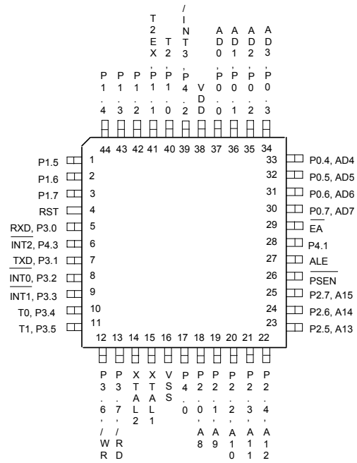
44-Pin QFP
