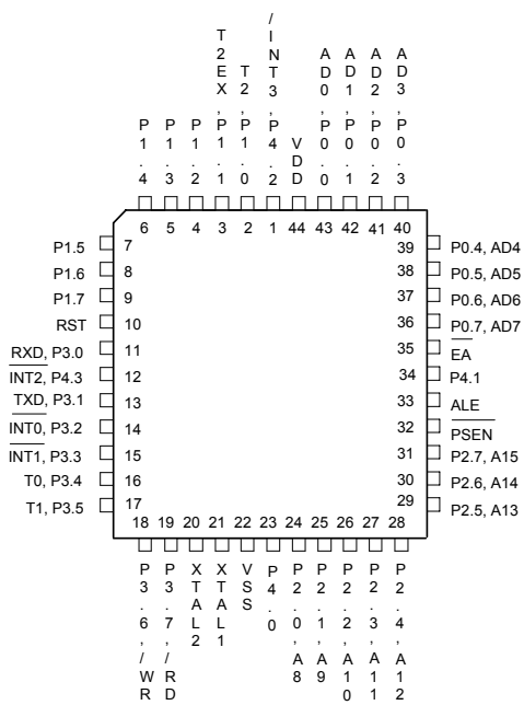
44-Pin PLCC
