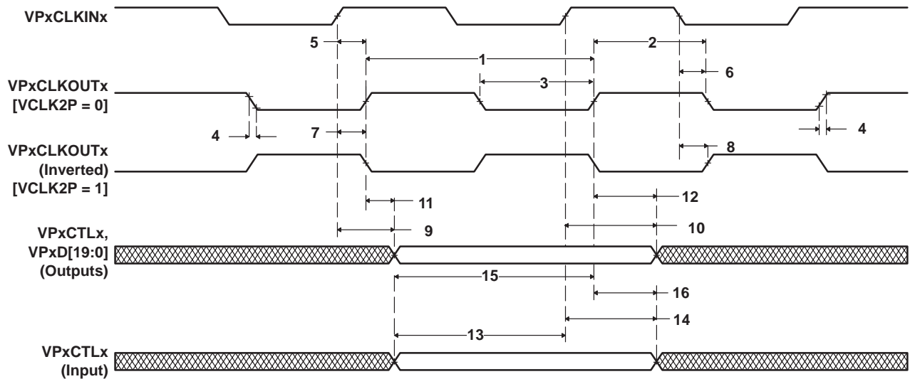
Figure 18–5. Video Port Display Data Output Timing and Control Input/Output Timing With Respect to VPxCLKINx and VPxCLKOUTx
