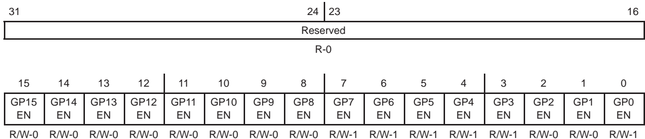
Figure 2–14. GPIO Enable Register (GPEN) [Hex Address: 01B0 0000]
