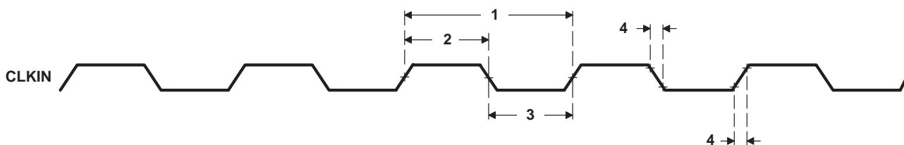
Figure 5–1. CLKIN Timing
