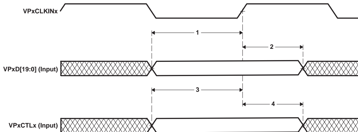
Figure 18–3. Video Port Capture Data and Control Input Timing
