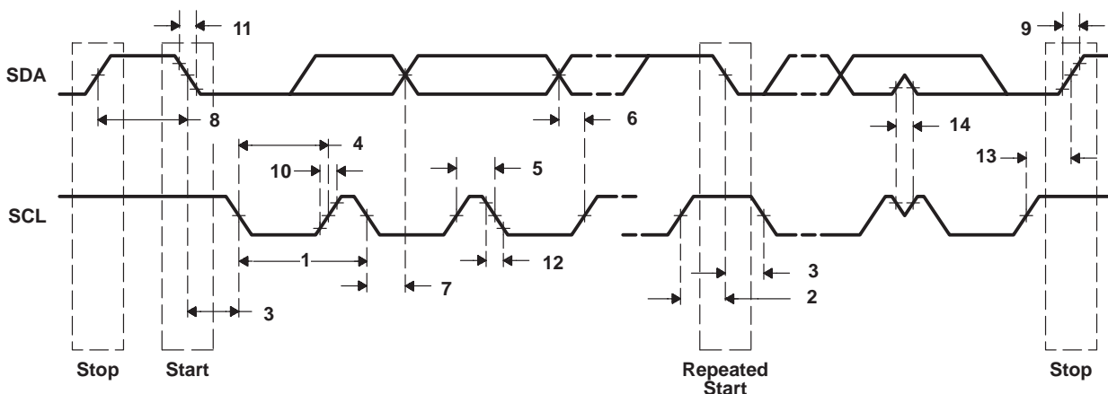
Figure 14–1. I2C Receive Timings
