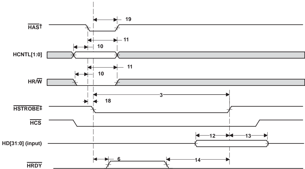
Figure 15–8. HPI32 Write Timing ( \overline{\text{HAS}} Used)
