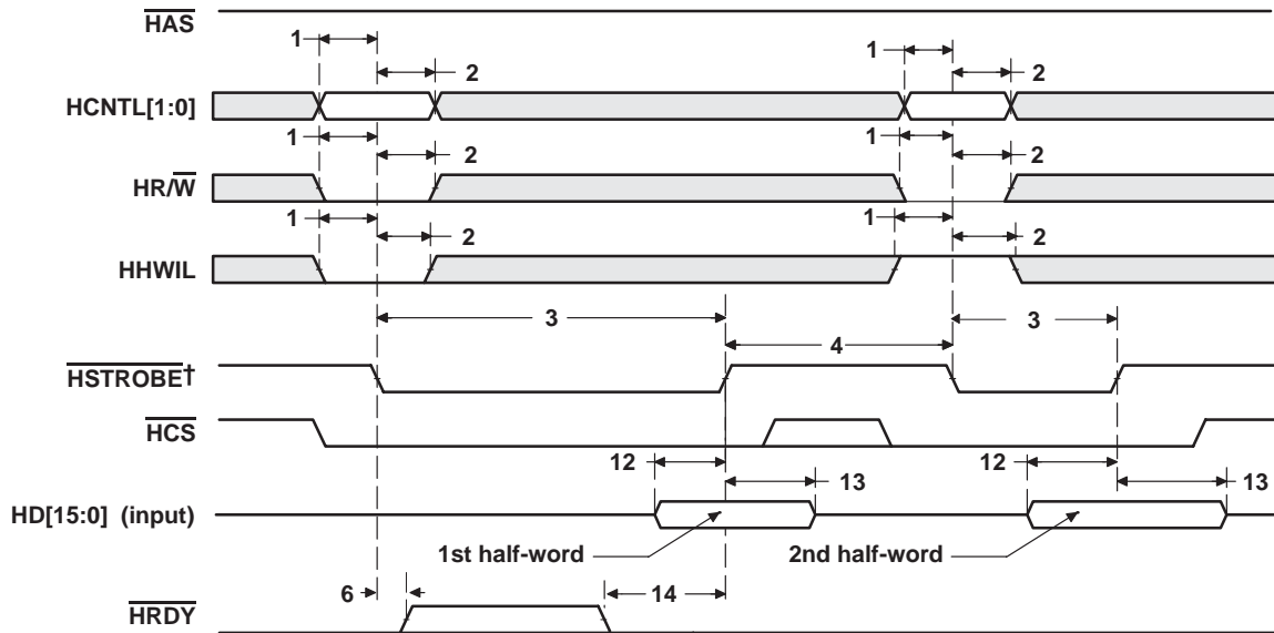
Figure 15–3. HPI16 Write Timing (HAS Not Used, Tied High)
