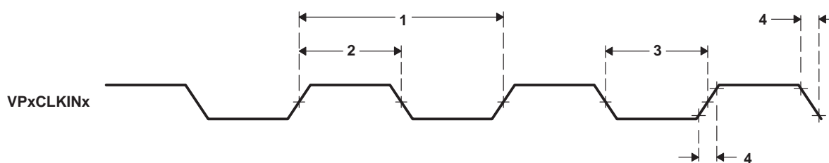
Figure 18–1. Video Port Capture VPxCLKINx Timing
