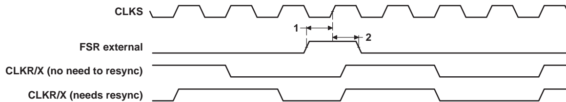
Figure 17-2. FSR Timing When GSYNC = 1
