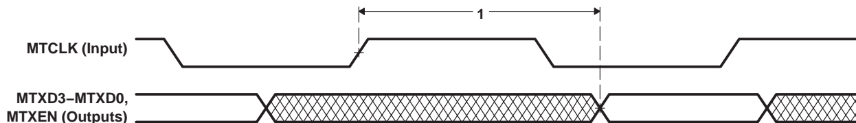
Figure 19–4. EMAC Transmit Interface Timing
