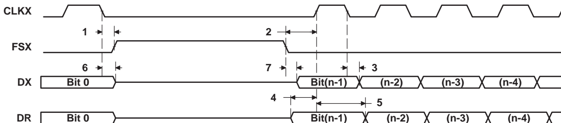
Figure 17–4. McBSP Timing as SPI Master or Slave: CLKSTP = 11b, CLKXP = 0
