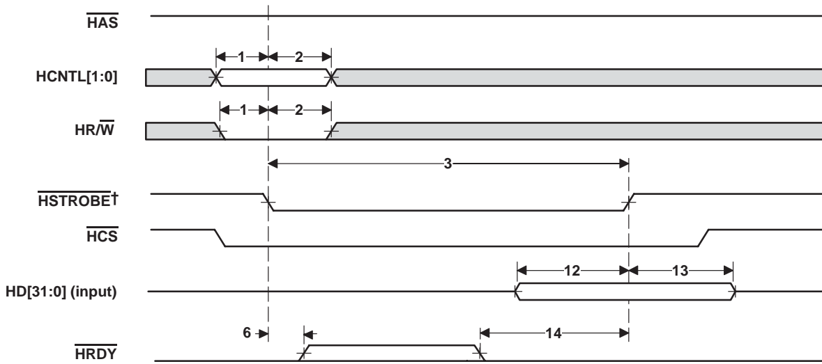
Figure 15–7. HPI32 Write Timing ( \overline{\text{HAS}} Not Used, Tied High)
