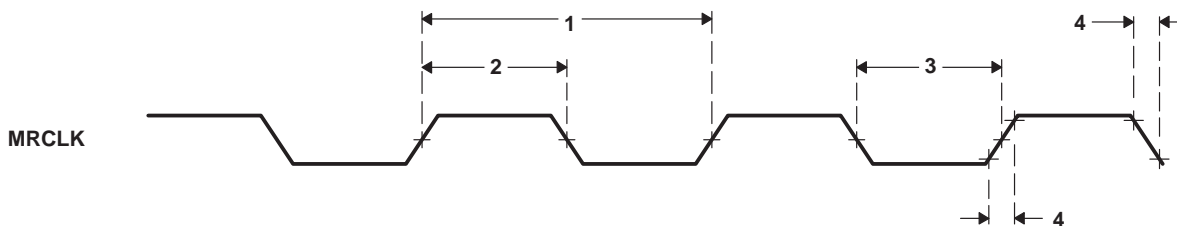
Figure 19–1. MRCLK Timing (EMAC – Receive)
