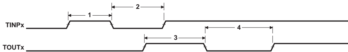
Figure 21–1. Timer Timing
