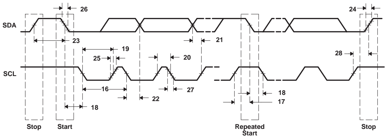
Figure 14–2. I2C Transmit Timings
