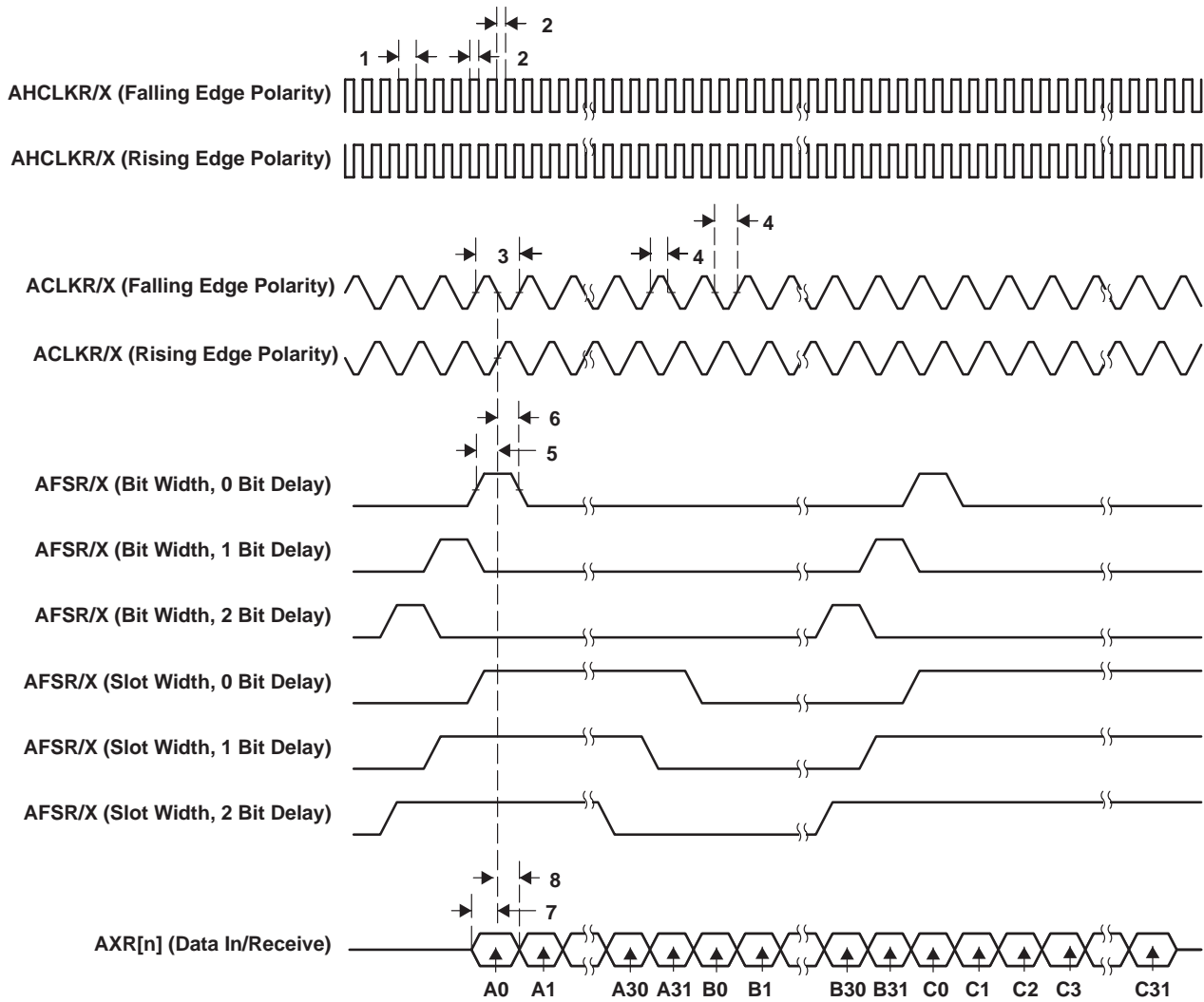
Figure 13-1. McASP Input Timings
