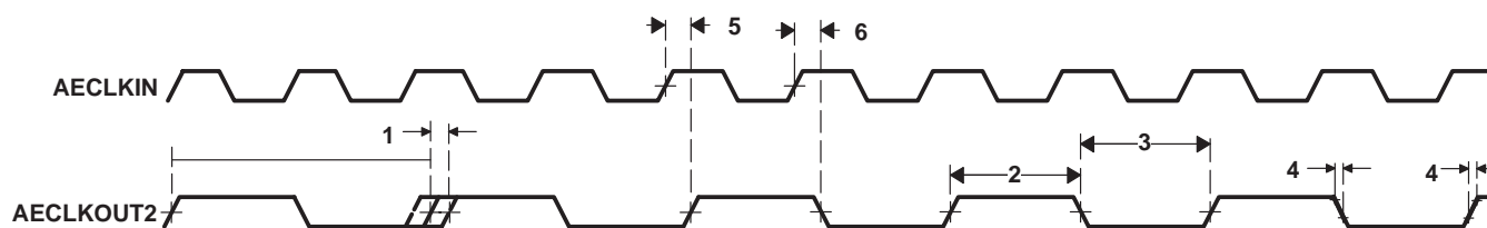
Figure 5–6. AECLKOUT2 Timing for the EMIFA Module
