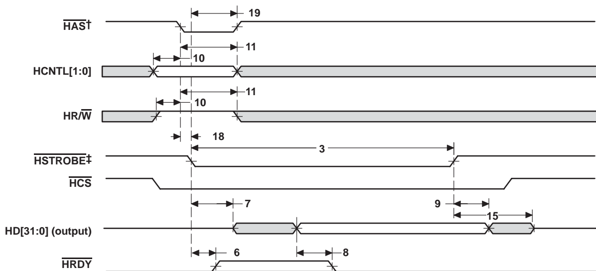
Figure 15–6. HPI32 Read Timing ( \overline{\text{HAS}} Used)
