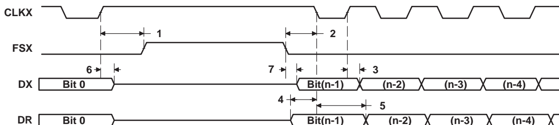
Figure 17–6. McBSP Timing as SPI Master or Slave: CLKSTP = 11b, CLKXP = 1
