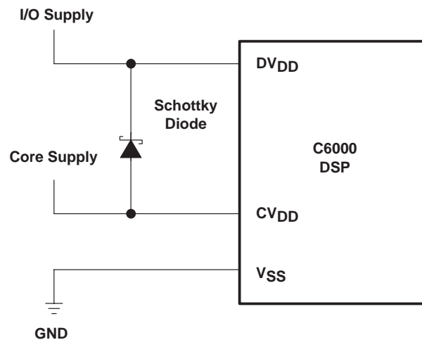
Figure 2–16. Schottky Diode Diagram
