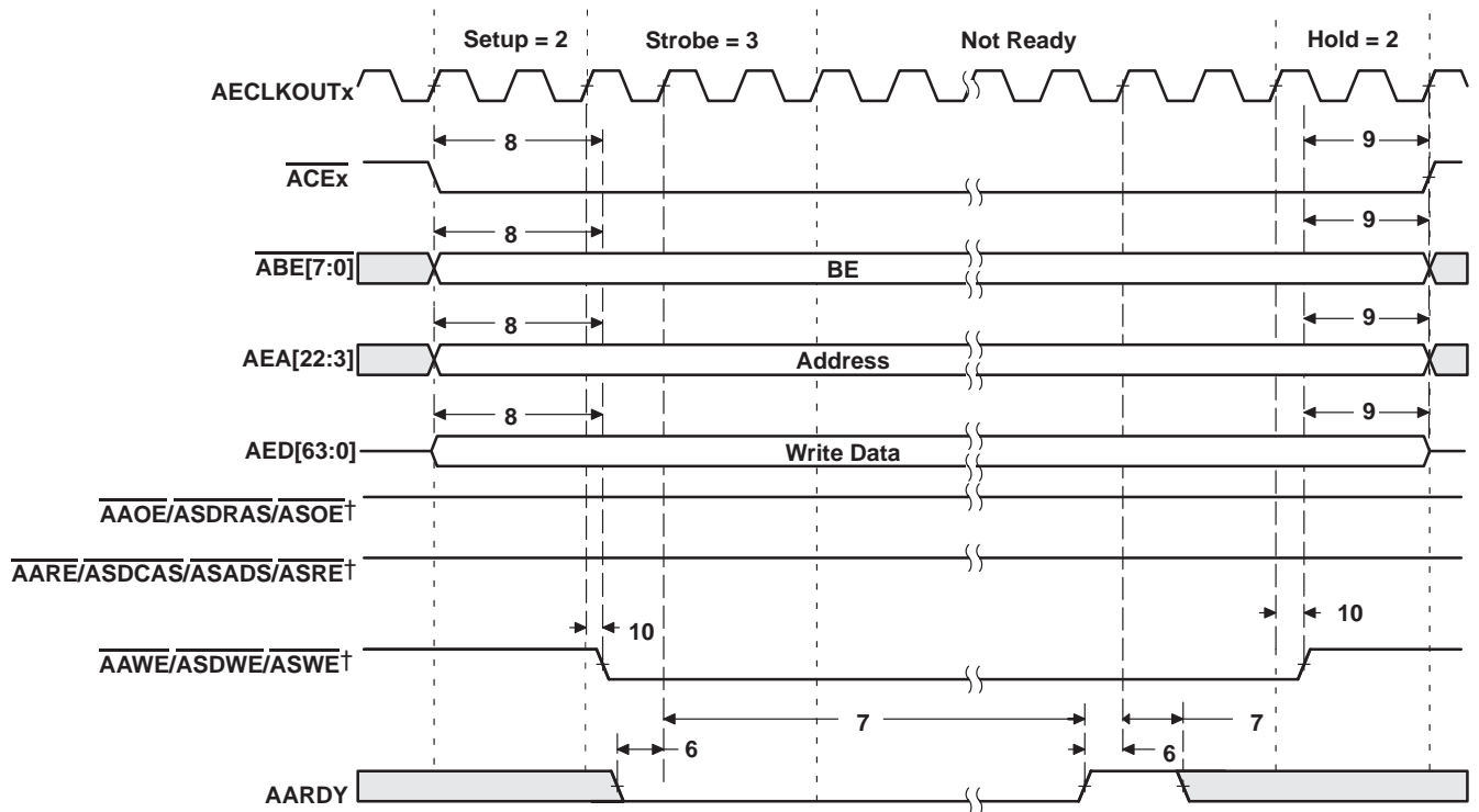
Figure 6–2. Asynchronous Memory Write Timing for EMIFA
