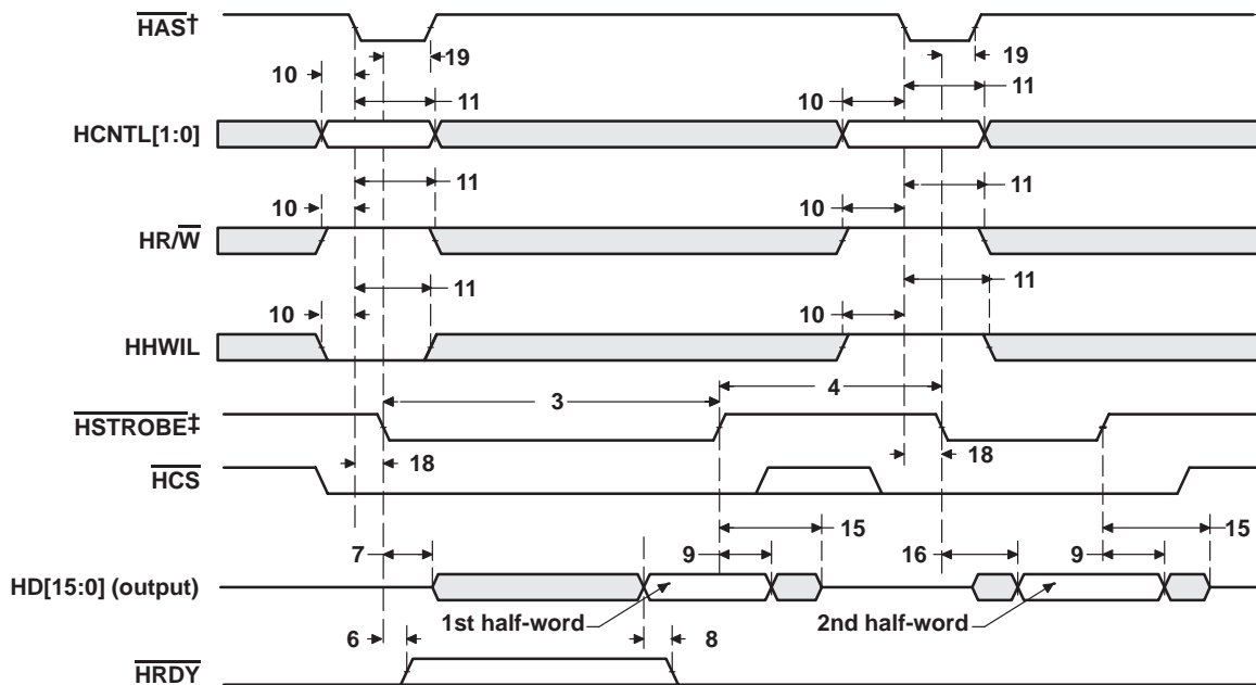
Figure 15–2. HPI16 Read Timing ( \overline{\text{HAS}} Used)
