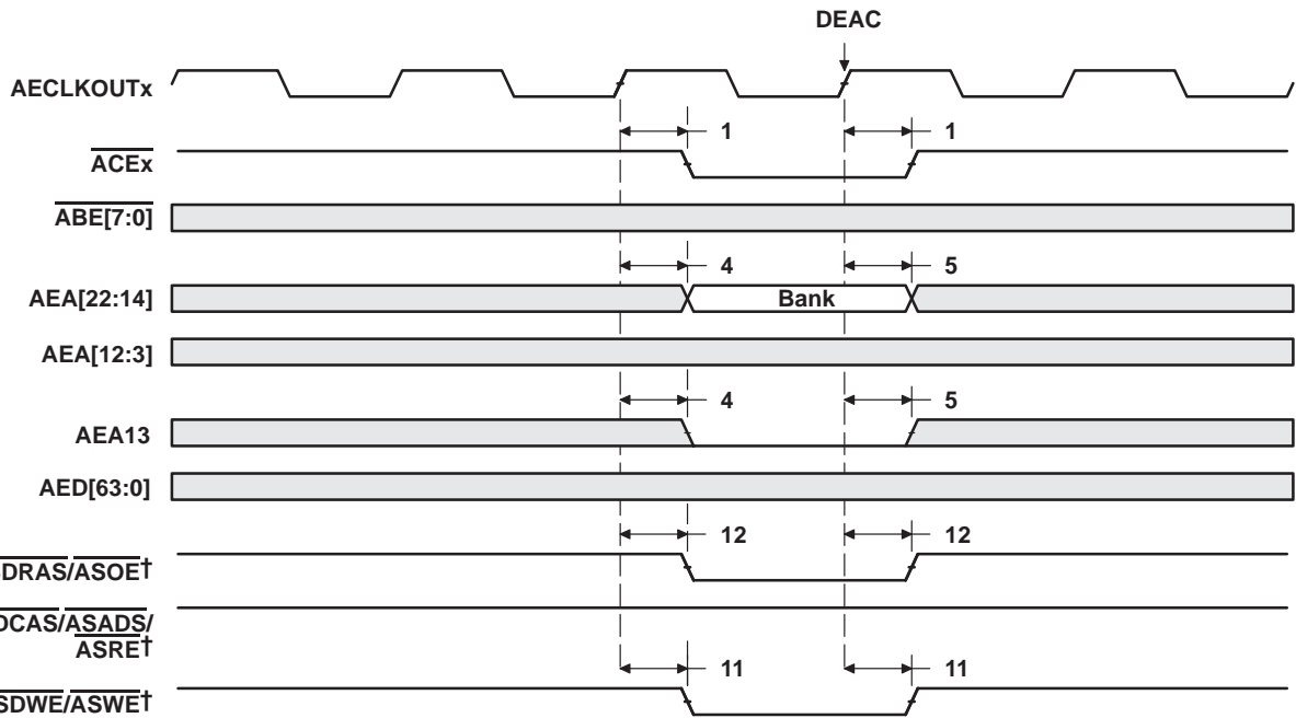
Figure 8-5. SDRAM DEAC Command for EMIFA
