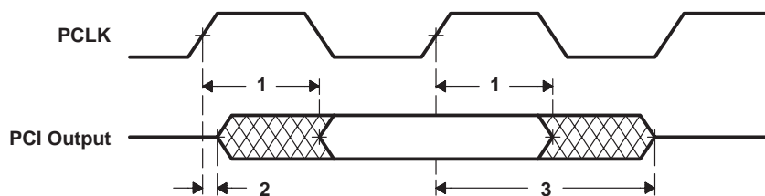
Figure 16–4. PCI Output Timing (33-/66-MHz)
