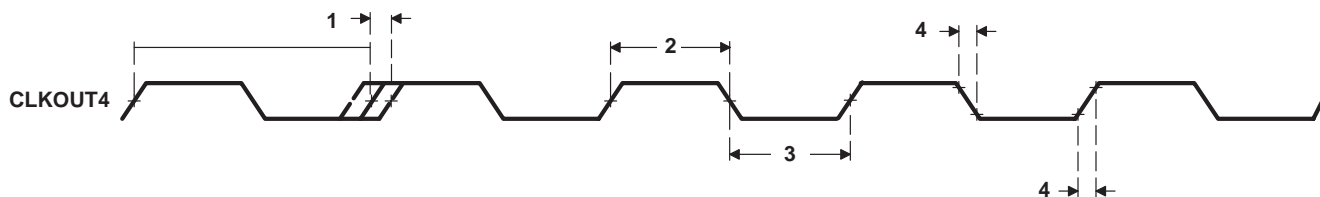
Figure 5–2. CLKOUT4 Timing
