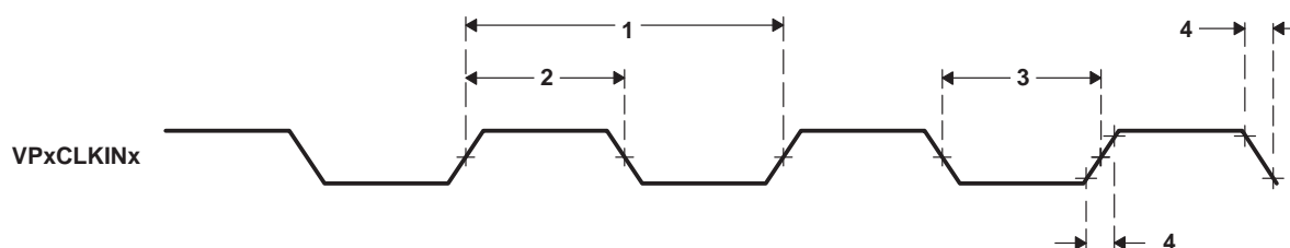
Figure 18–4. Video Port Display VPxCLKINx Timing
