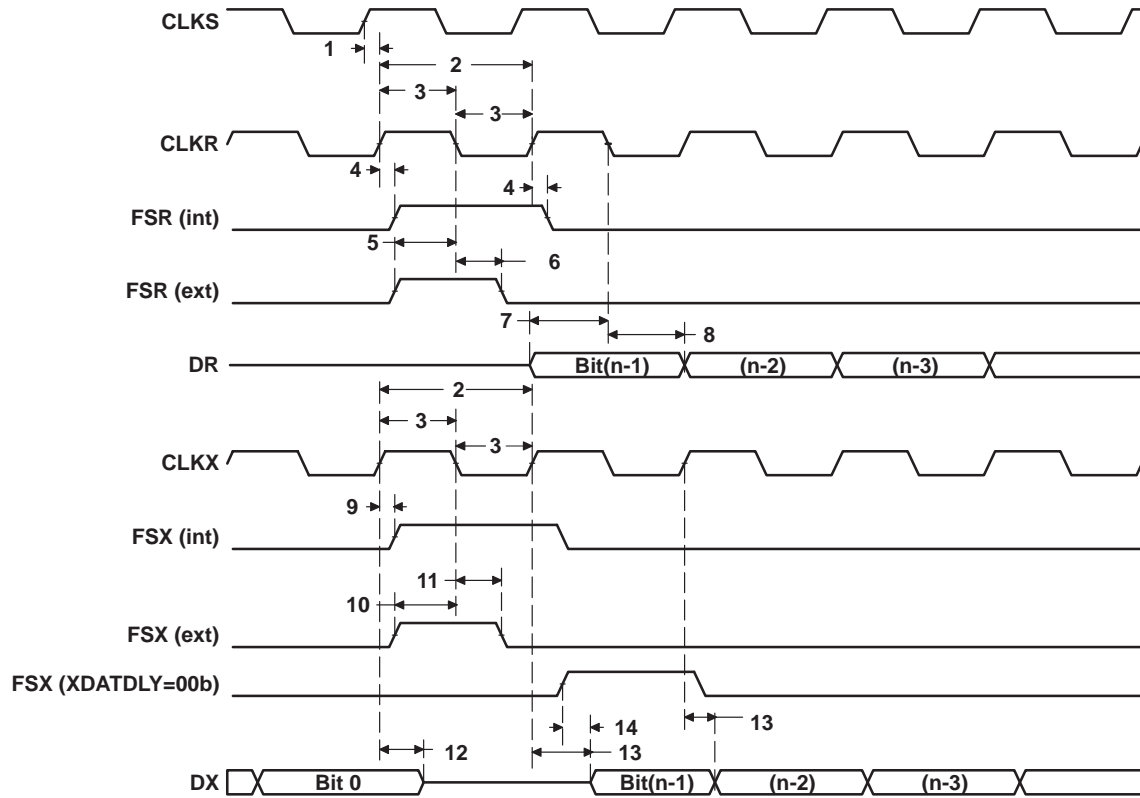
Figure 17-1. McBSP Timing
