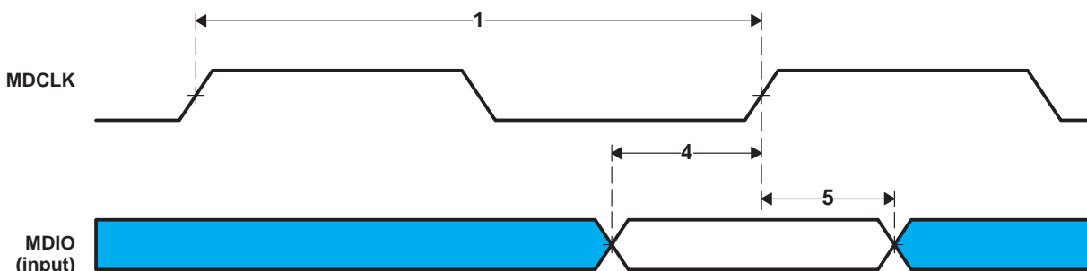
Figure 20–1. MDIO Input Timing
