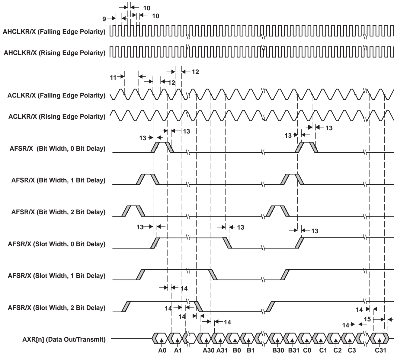
Figure 13–2. McASP Output Timings
