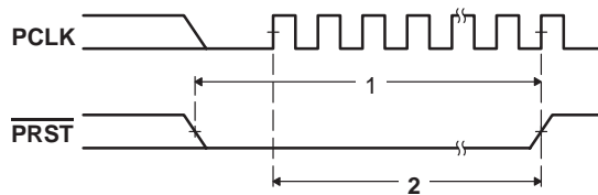
Figure 16–2. PCI Reset ( \overline{\text{PRST}} ) Timing
