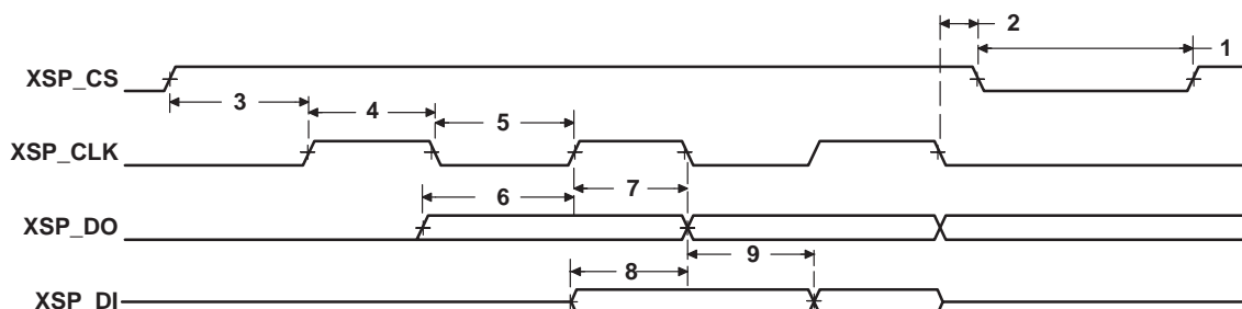
Figure 16–5. PCI Serial EEPROM Interface Timing
