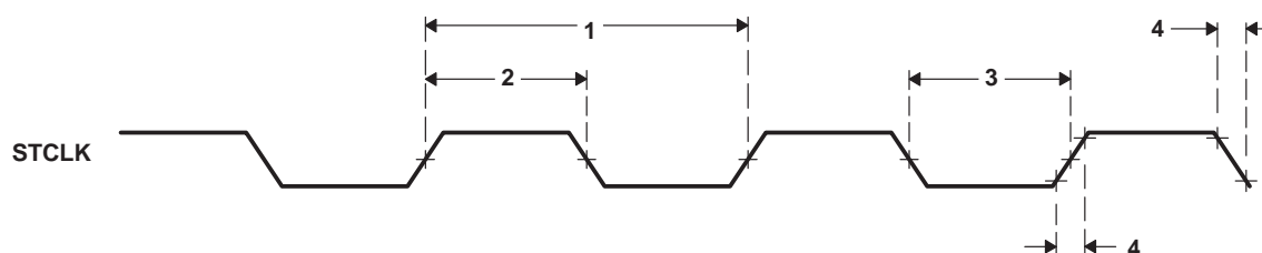
Figure 18–2. STCLK Timing
