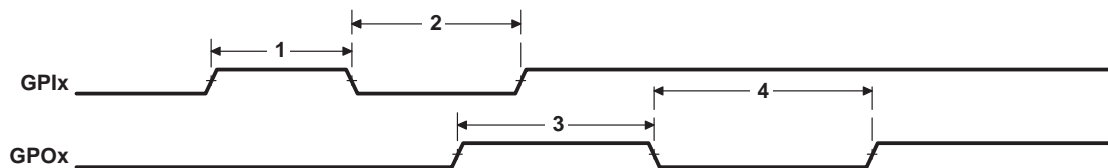
Figure 22–1. GPIO Port Timing
