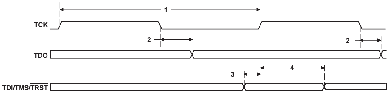
Figure 23–1. JTAG Test-Port Timing
