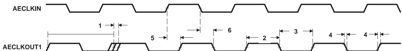
Figure 5–5. AECLKOUT1 Timing for the EMIFA Module
