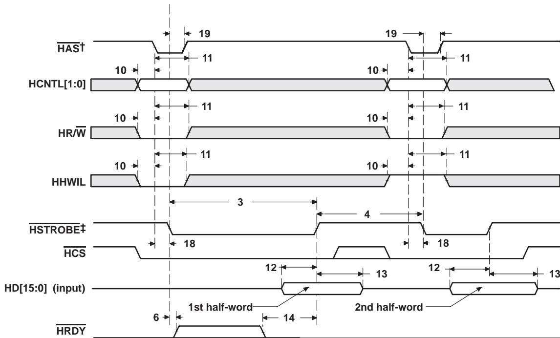
Figure 15–4. HPI16 Write Timing (HAS Used)
