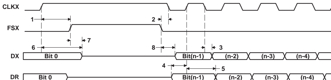
Figure 17–5. McBSP Timing as SPI Master or Slave: CLKSTP = 10b, CLKXP = 1
