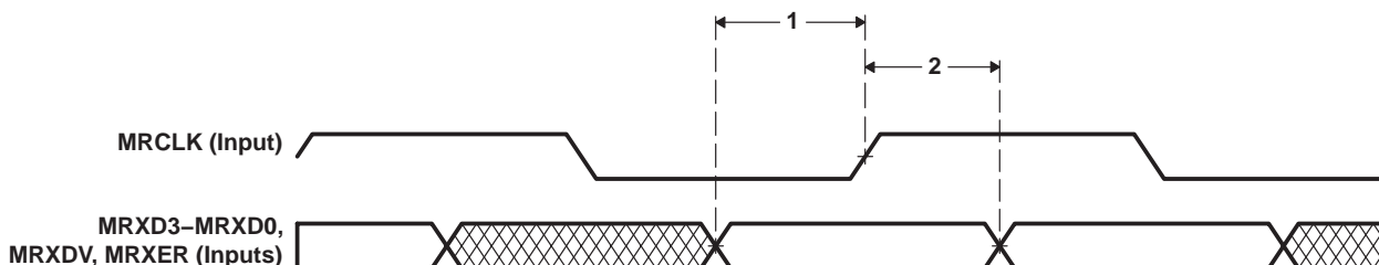
Figure 19–3. EMAC Receive Interface Timing
