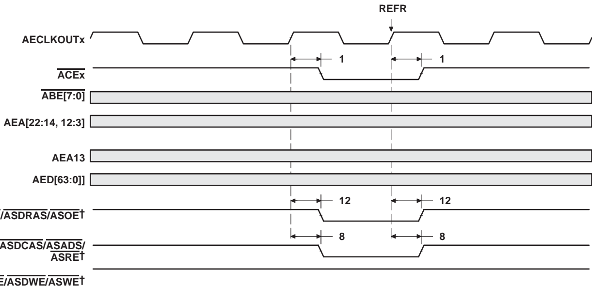
Figure 8-6. SDRAM REFR Command for EMIFA
