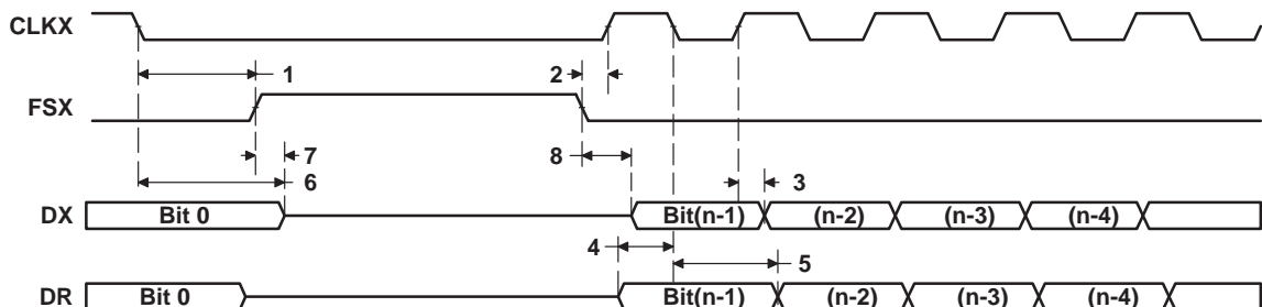
Figure 17–3. McBSP Timing as SPI Master or Slave: CLKSTP = 10b, CLKXP = 0
