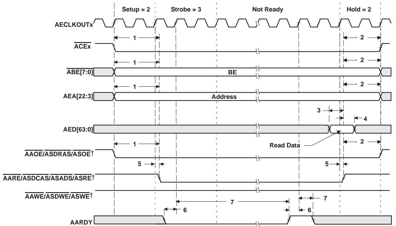
Figure 6–1. Asynchronous Memory Read Timing for EMIFA
