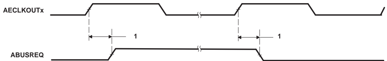
Figure 10–1. BUSREQ Timing for EMIFA
