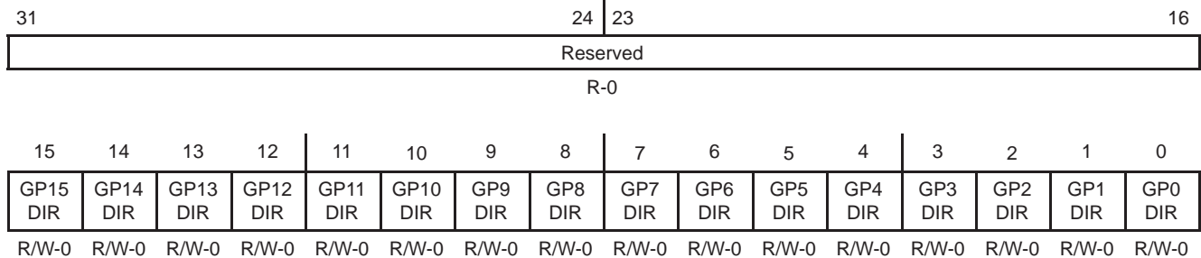
Figure 2–15. GPIO Direction Register (GPDIR) [Hex Address: 01B0 0004]
