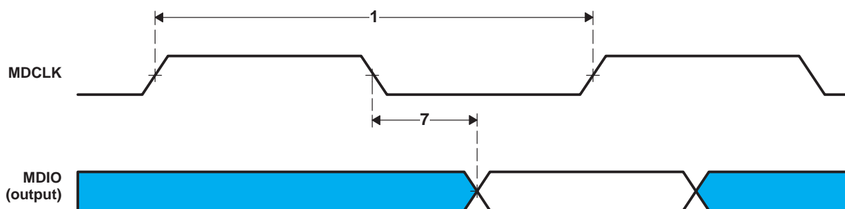
Figure 20–2. MDIO Output Timing
