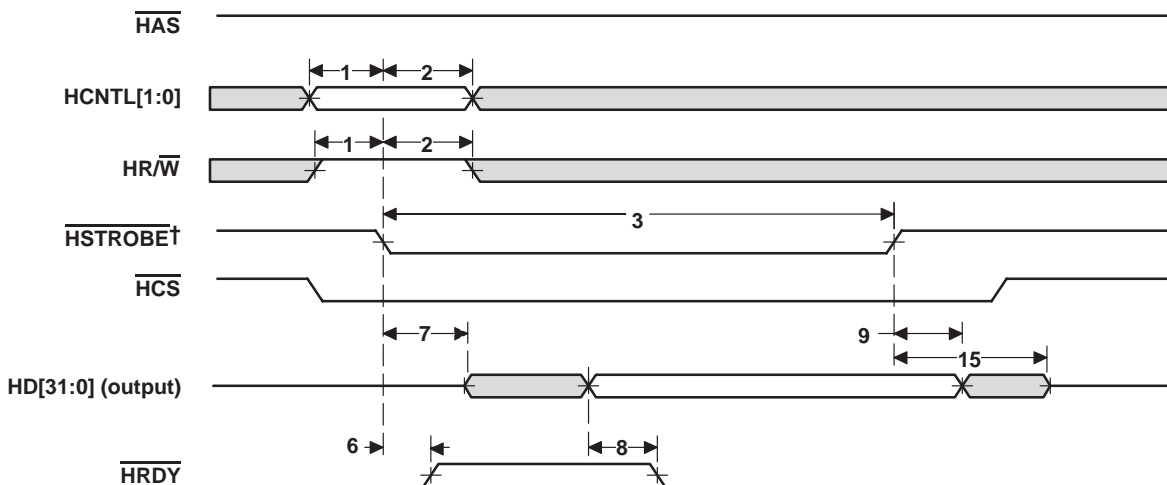
Figure 15–5. HPI32 Read Timing ( \overline{\text{HAS}} Not Used, Tied High)
