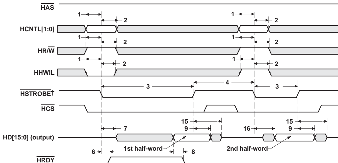
Figure 15–1. HPI16 Read Timing ( \overline{\text{HAS}} Not Used, Tied High)
