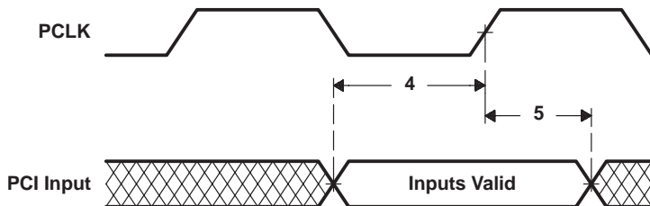
Figure 16–3. PCI Input Timing (33-/66-MHz)
