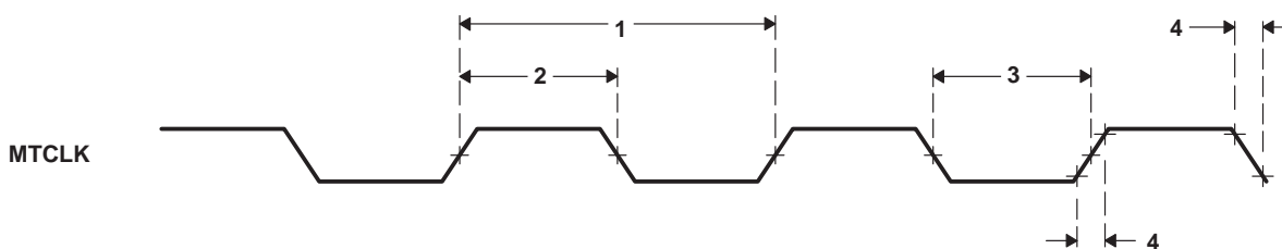
Figure 19–2. MTCLK Timing (EMAC – Transmit)
