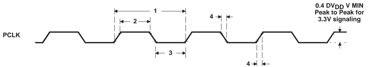
Figure 16–1. PCLK Timing
