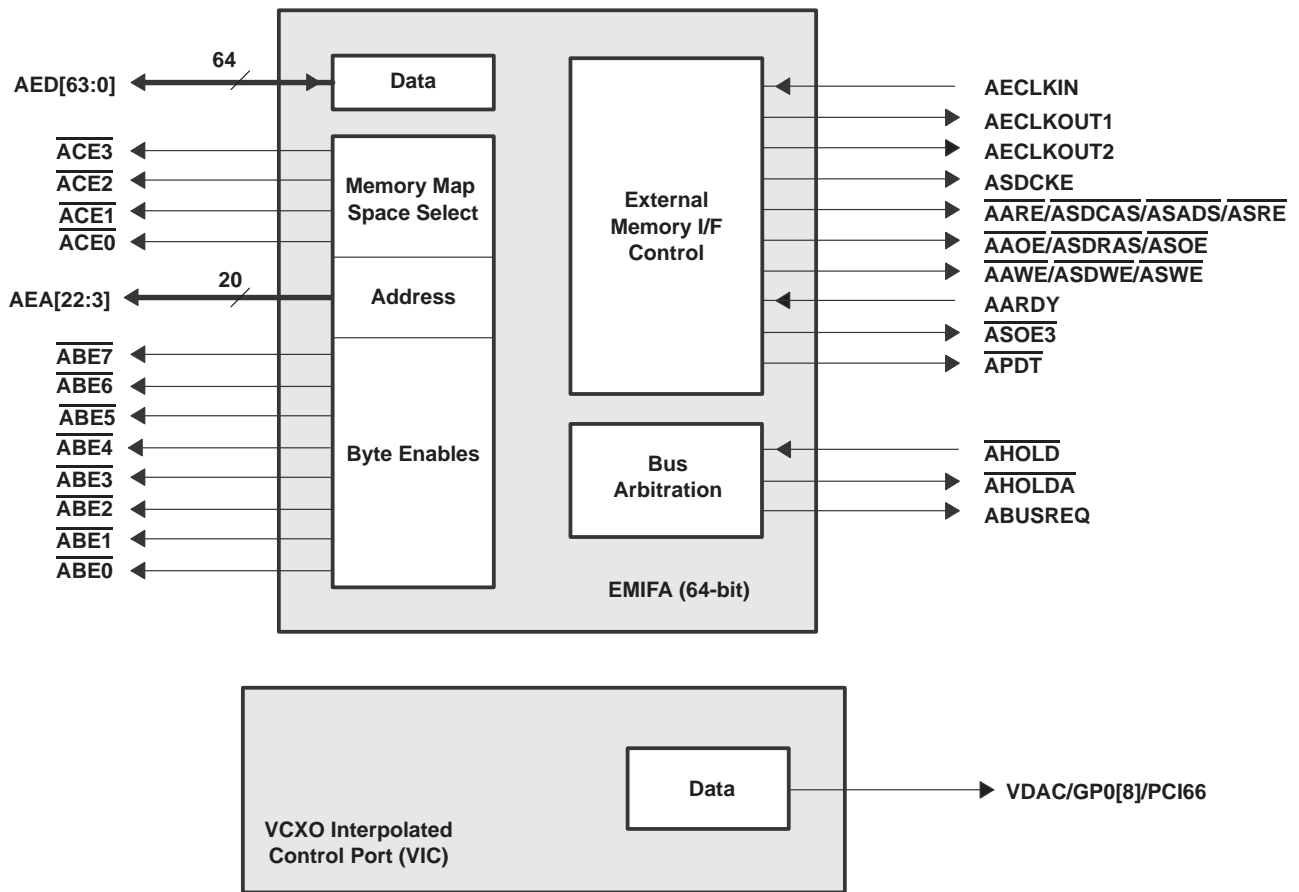
Figure 1-6. Peripheral Signals
