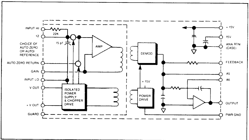
'A Isolation Amplifier Functional Block Diagram.
