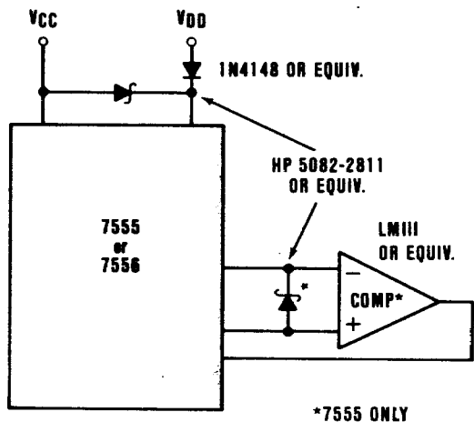
Figure 5. Diode Protection
