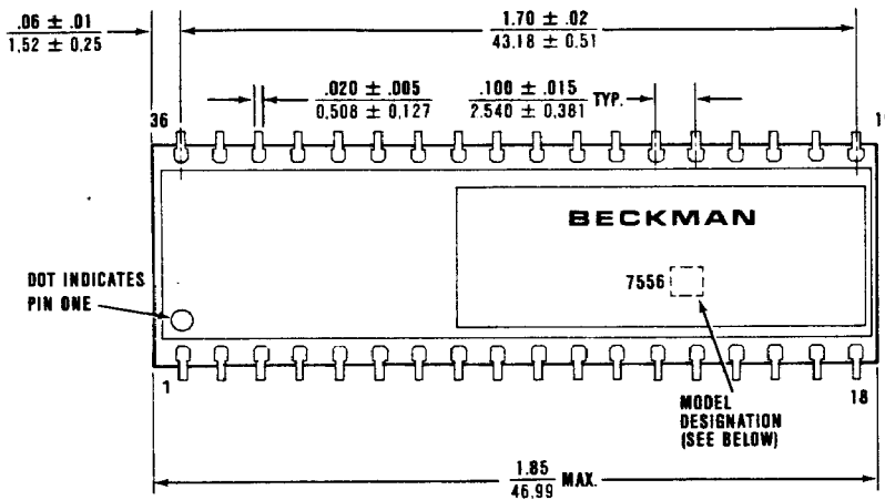
Outline Drawing—Series 7556
