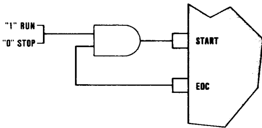
Figure 13. RUN/STOP Operation
