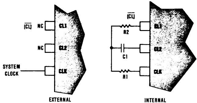
Figure 9. Cloning Configurations
