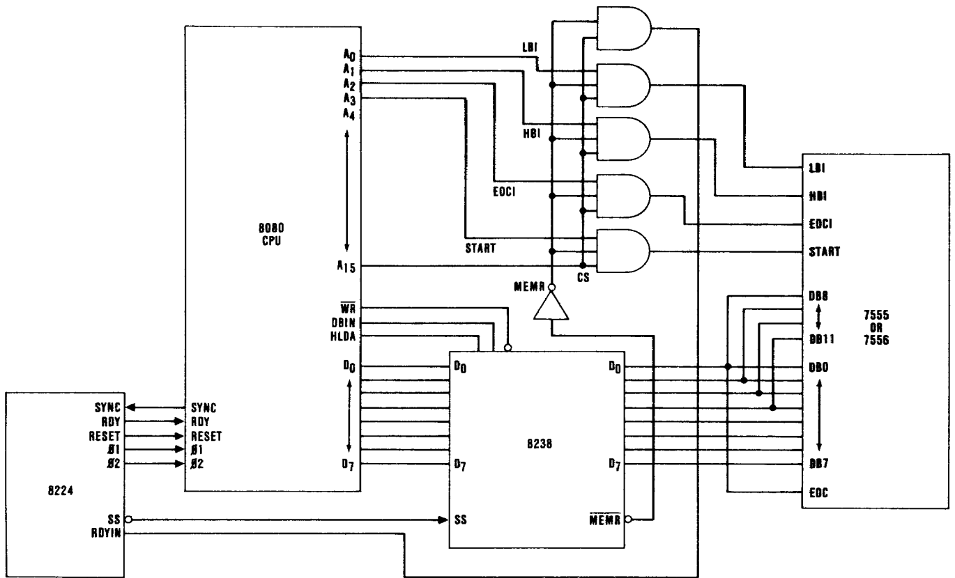
Figure 22. CPU Interface Configuration
