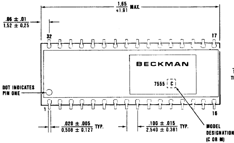
Outline Drawing—Series 7555
