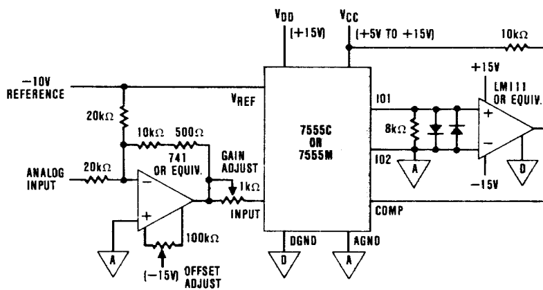
Figure 19. Bipolar Operation (7555)
