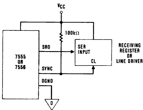
Figure 17. Serial Data Transfer
