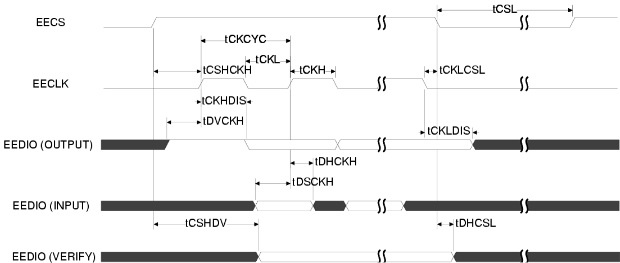
Figure 6.7 EEPROM Timing
