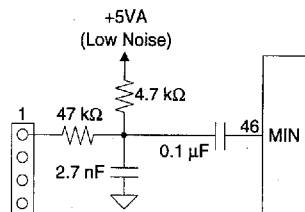
Figure 4. Mono Input
