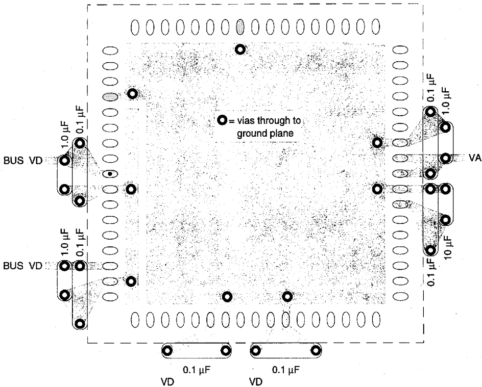
Figure 17. Recommended Decoupling Capacitor Positions
