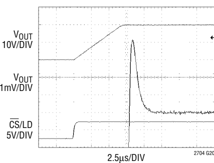
Settling ±10V
