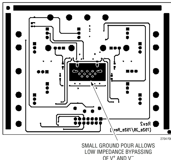
Figure 6. DC752A Routing, Bypass
