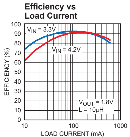
Figure 4— V_{IN} = 2.5V to 6V , V_{OUT} = 1.8V , I_{LOAD} = 600mA Step-Down Circuit (L = 10µH for Higher Light-Load Efficiency)
