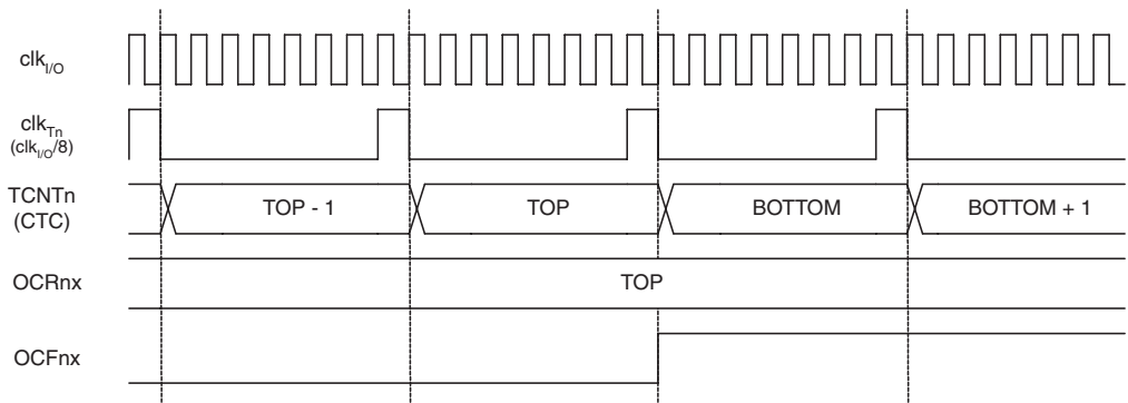
Figure 13-13. Timer/Counter Timing Diagram, Clear Timer on Compare mode, with Prescaler ( f_{clk\_I/O}/8 )
