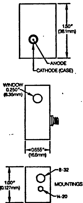
TO-3/3
