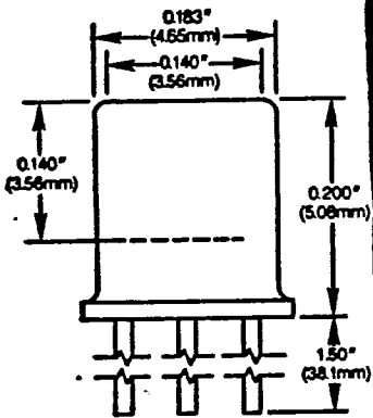
TO-18
