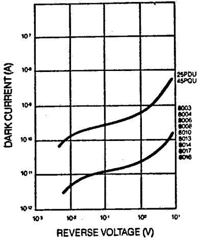
DARK CURRENT vs. VOLTAGE
