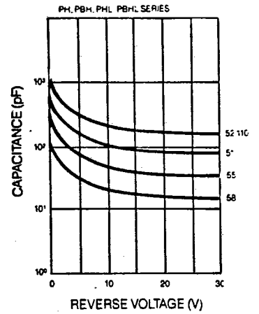
CAPACITANCE vs. VOLTAGE
