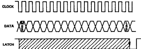
Figure 7. Signal Requirements of AD1856
