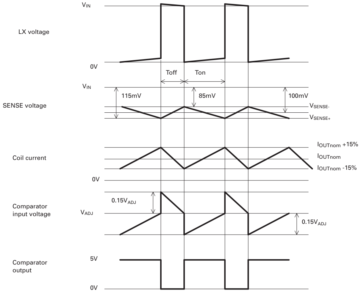
Figure 1 Operating waveforms
