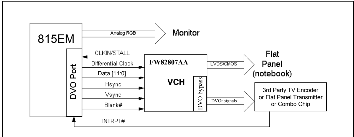
Figure 9. Digital Video Out Port Mobile Application Block Diagram With VCH
