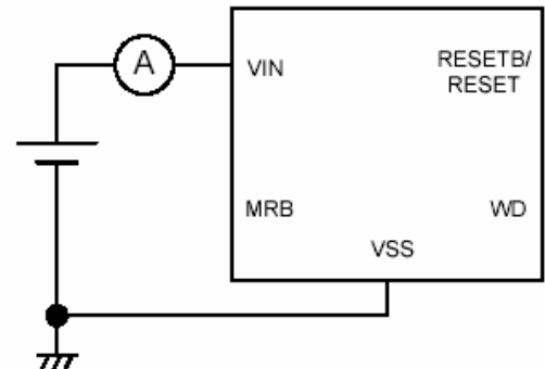
Circuit 2
