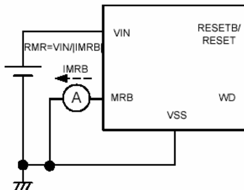
Circuit 11
