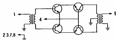
Figure 10. Functional Schematic
