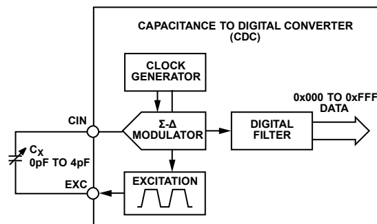
Figure 21. CDC Simplified Block Diagram
