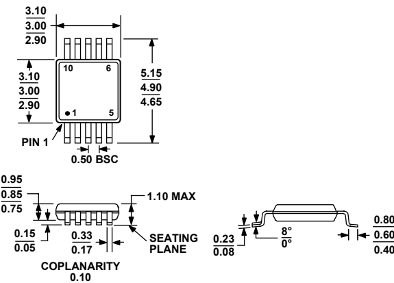
Figure 52. 10-Lead Mini Small Outline Package [MSOP] (RM-10)
