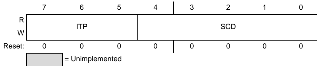
Figure 18. Low Power Configuration Register
