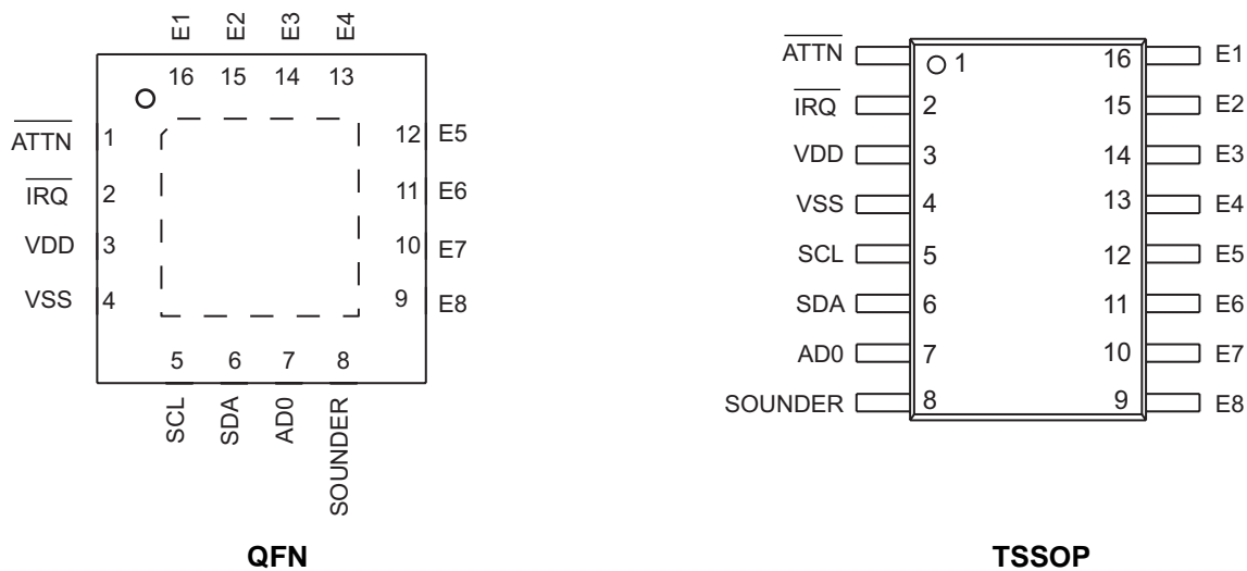
Figure 3. Package Pinouts
