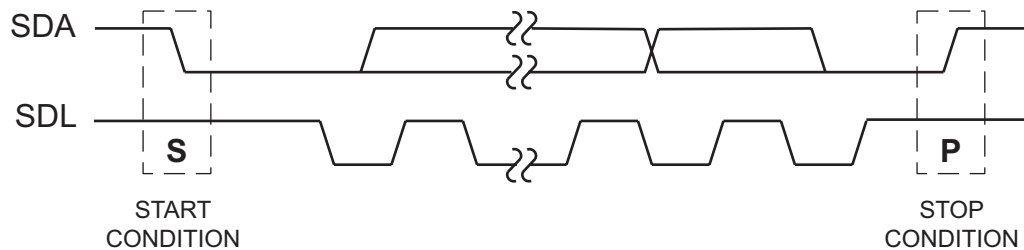
Figure 7. Bit Transfer
