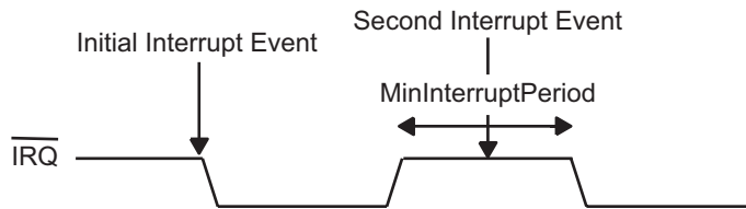
Figure 22. \overline{\text{IRQ}} Timing Diagram - Case 1
