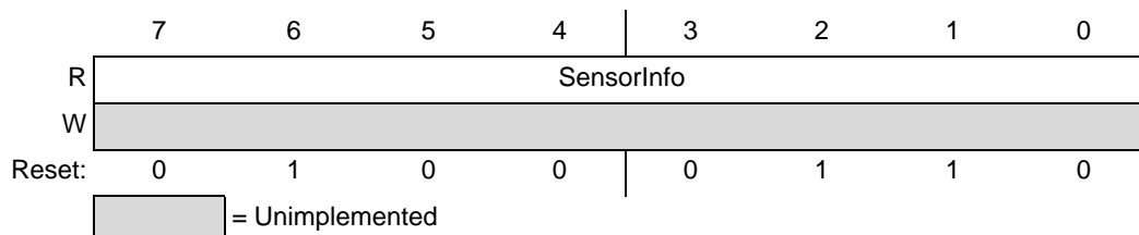
Figure 27. Sensor Information Register
