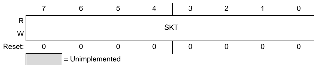
Figure 24. Stuck Key Timeout Register
