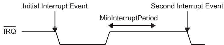
Figure 23. \overline{\text{IRQ}} Timing Diagram - Case 2
