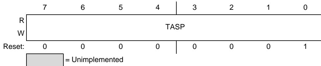
Figure 14. Touch Acquisition Sample Period Register
