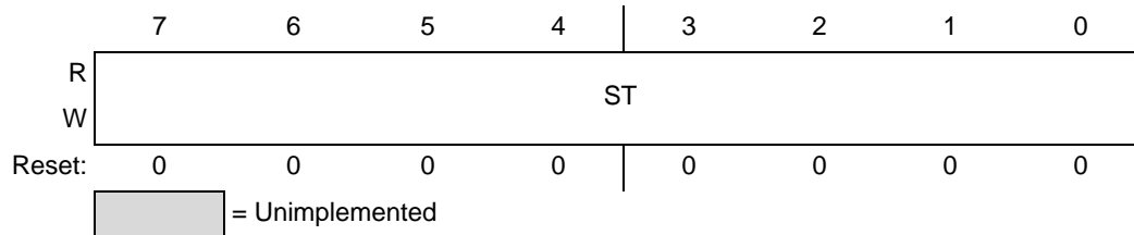
Figure 25. Sensitivity Threshold Register
