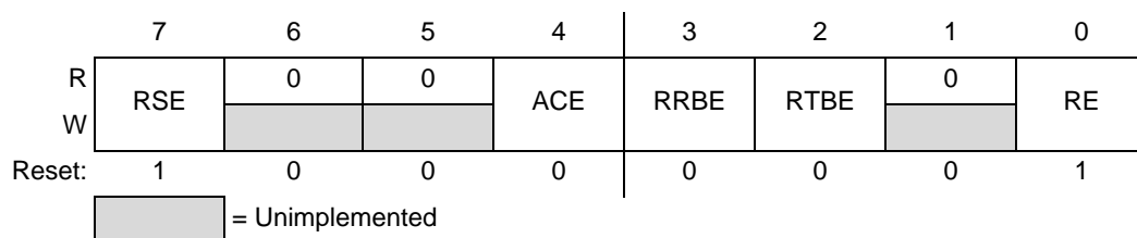
Figure 13. Rotary Configuration Register
