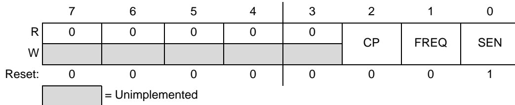
Figure 26. Sounder Configuration Register
