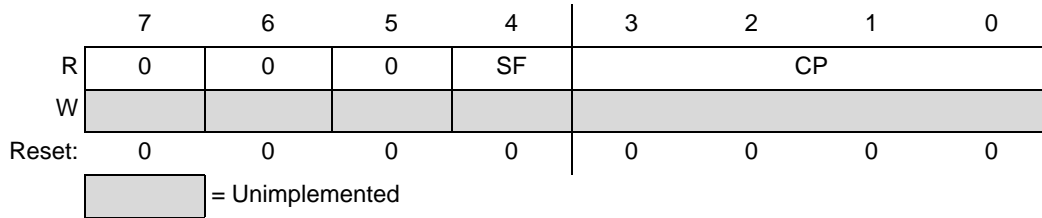
Figure 19. Rotary Status Register
