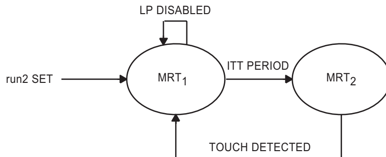
Figure 17. Low Power Scan Period Transition Diagram
