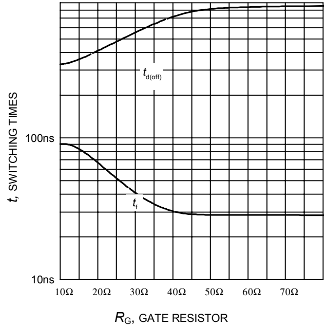
Figure 10. Typical switching times as a function of gate resistor (inductive load, T_J=175^{\circ}\text{C} , V_{CE}=600\text{V} , V_{GE}=0/15\text{V} , I_C=15\text{A} , Dynamic test circuit in Figure E)
