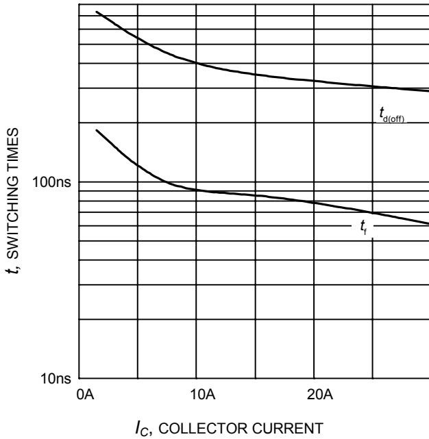
Figure 9. Typical switching times as a function of collector current (inductive load, T_J=175^{\circ}\text{C} , V_{CE}=600\text{V} , V_{GE}=0/15\text{V} , R_G=14.8\Omega , Dynamic test circuit in Figure E)
