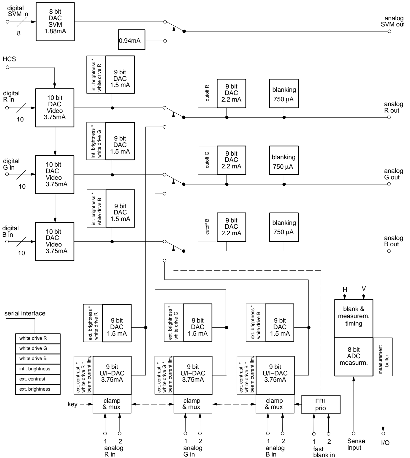
Fig. 2-27: Analog back-end
