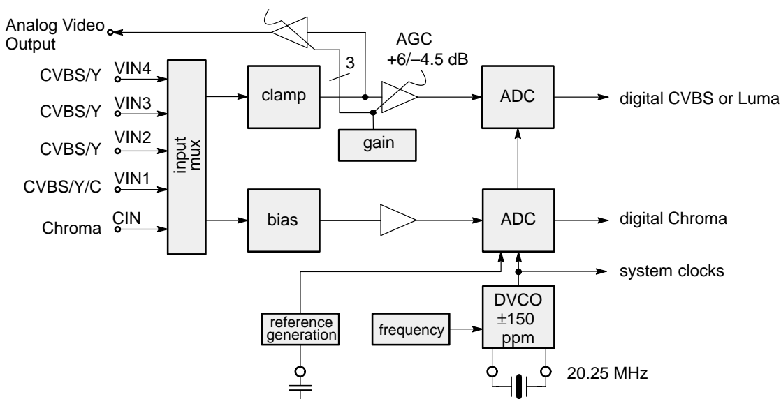
Fig. 2–1: Analog front-end
