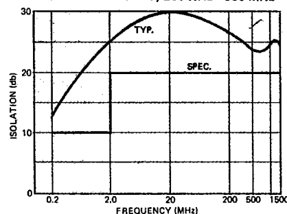
MODELS PSP-210, PSF-210 - 2 OUTPUT, 200 KHz - 800 MHz
