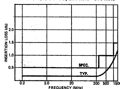
MODELS PSP-210, PSF-210 - 2 OUTPUT, 200 KHz - 800 MHz
