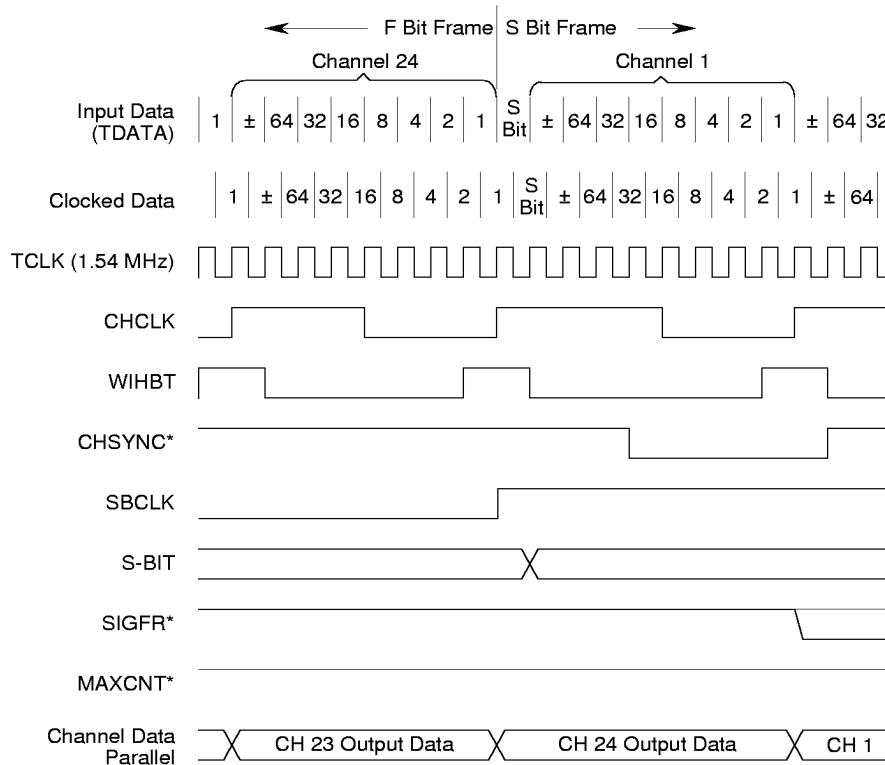
Figure 2. Signal Relationships at Beginning of F 3 Frame (S-BIT).
