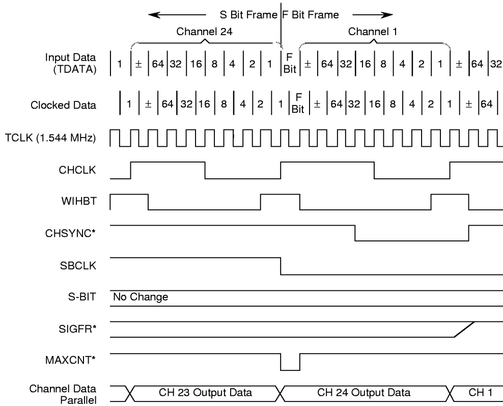
Figure 3. Signal Relationship During Frame Alarm and Search for Resynchronization.
