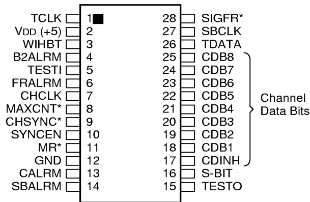
Figure 1. Pin Configuration.
