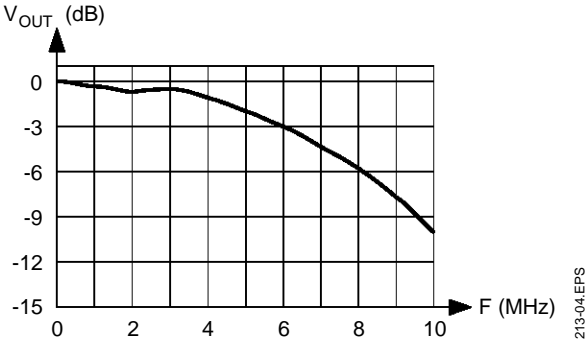
Figure 1 : Output Signal Bandwidth without Video peaking
