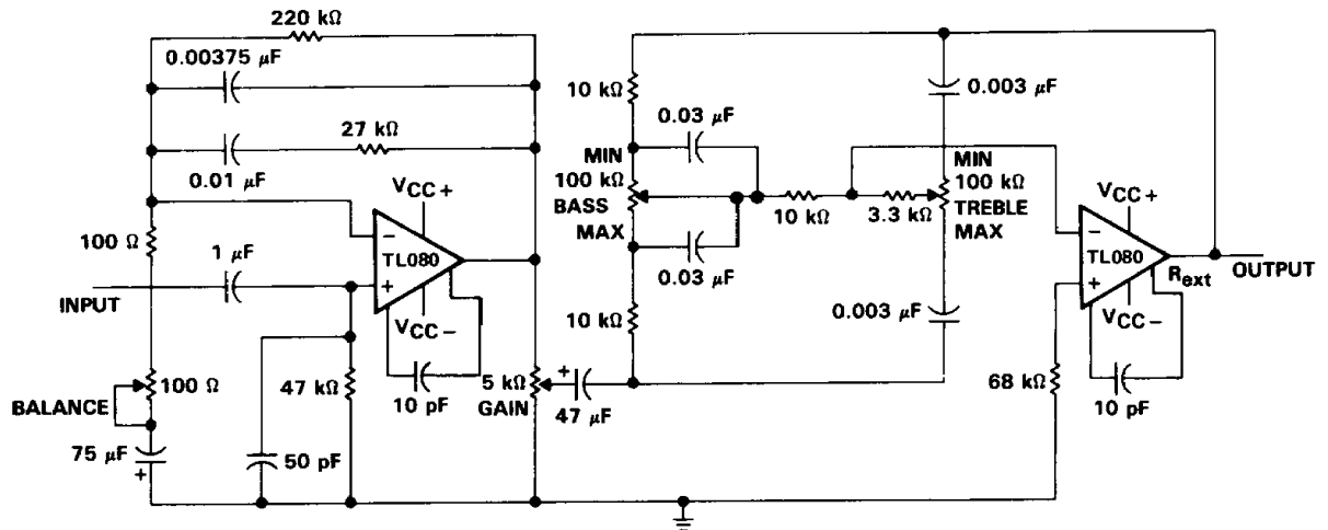
FIGURE 29. IC PREAMPLIFIER
