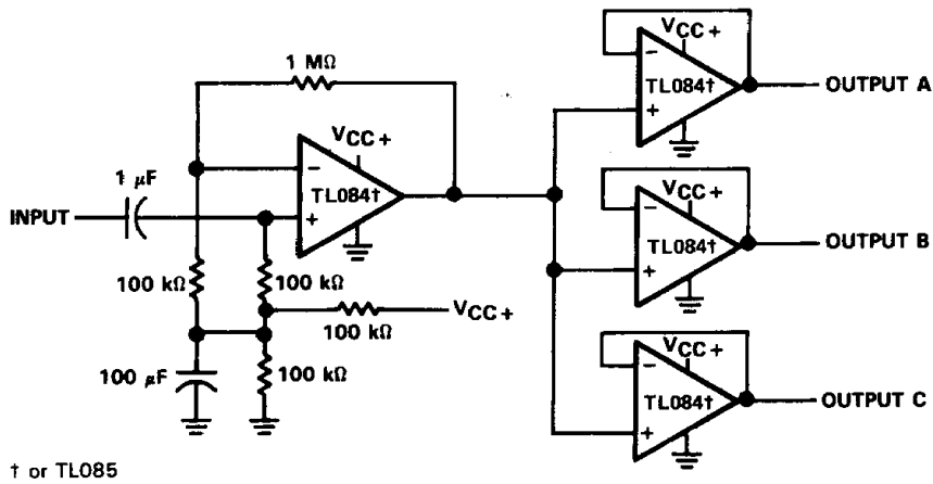
FIGURE 26. AUDIO DISTRIBUTION AMPLIFIER
