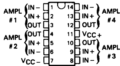
TL085 N PACKAGE
