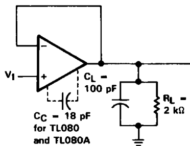
FIGURE 1. UNITY-GAIN AMPLIFIER
