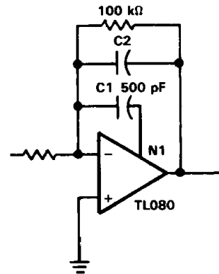
FIGURE 3. FEED-FORWARD COMPENSATION
