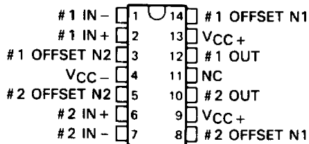
TL083, TL083A D, J, OR N PACKAGE (TOP VIEW)
