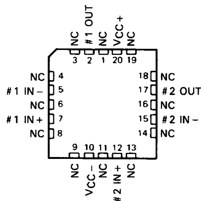
TL082M . . . FK CHIP CARRIER PACKAGE (TOP VIEW)
