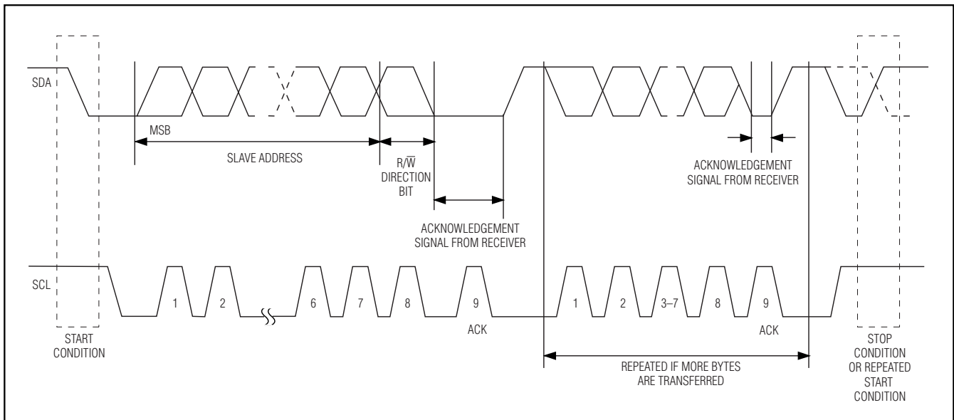
Figure 3. Data Transfer Protocol
