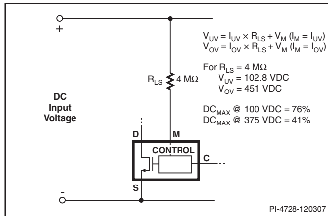
Figure 30. Line Sensing for Undervoltage, Overvoltage and Line Feed-Forward.
