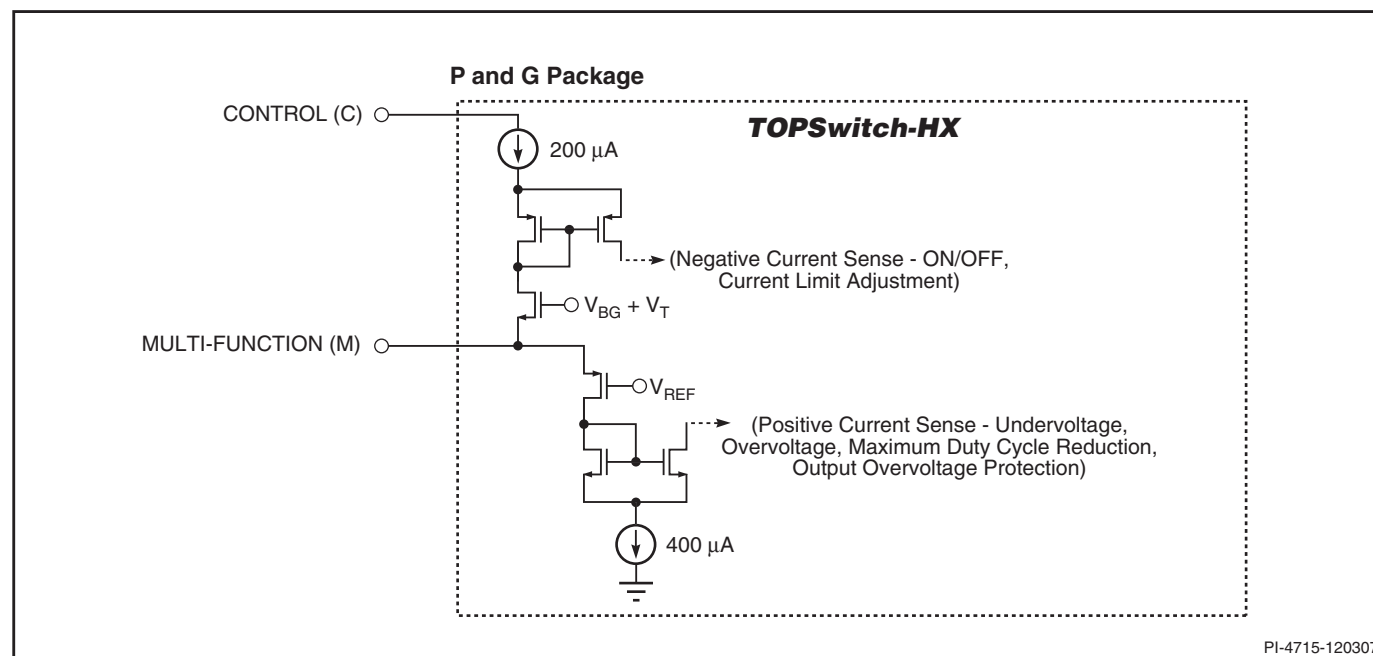
Figure 13b. MULTI-FUNCTION (M) Pin Input Simplified Schematic.
