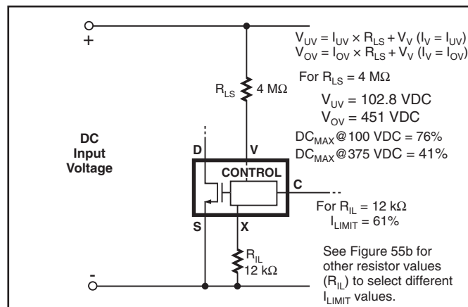
Figure 5. TOP254-258 Y and All M/E Package Line Sense and Externally Set Current Limit.
