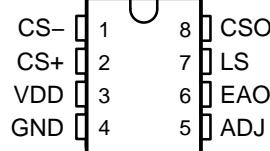
PDIP (P) PACKAGE (TOP VIEW)
