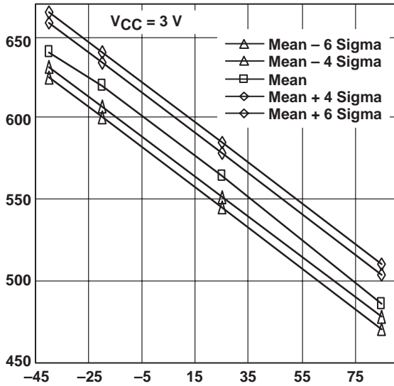
Figure 4. V_{(RefVT)} vs Temperature, V_{CC} = 3\text{ V}
