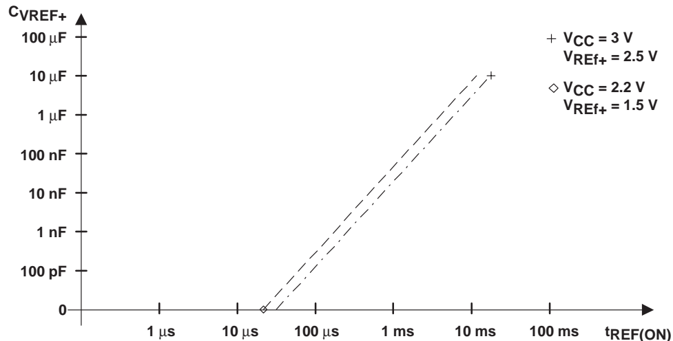
Figure 11. Maximum Settling Time of Internal Reference t_{REF(ON)} vs External Capacitor on V_{REF+}
