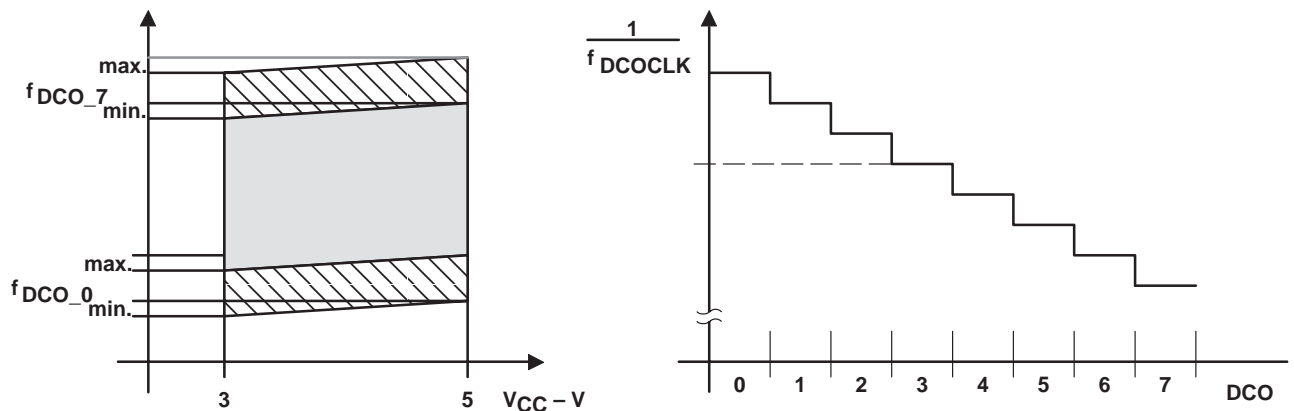
Figure 10. DCO Characteristics
