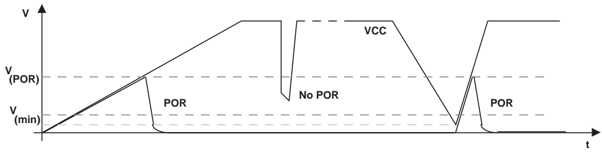
Figure 8. Power-On Reset (POR) vs Supply Voltage
