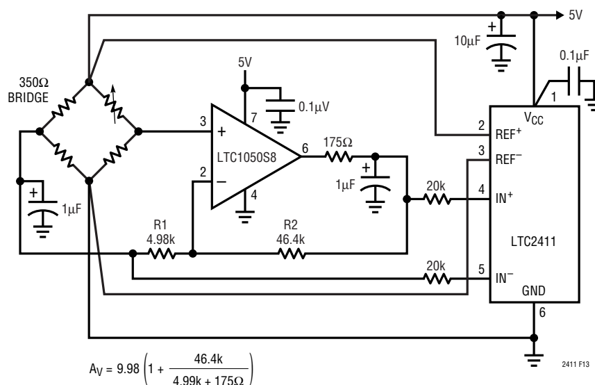
Figure 13. Bridge Amplification Using a Single Amplifier
