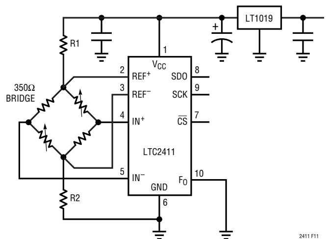
2411 F11 R1 AND R2 CAN BE USED TO INCREASE TOLERABLE AC COMPONENT ON REF SIGNALS
