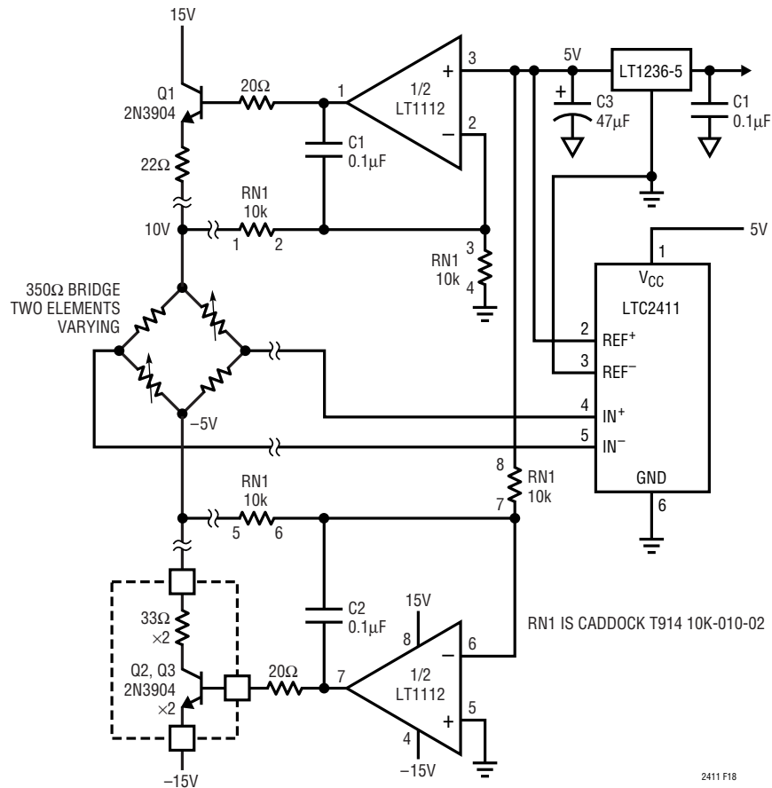
Figure 18. Use Resistor Arrays to Provide Precise Matching in Excitation Amplifier
