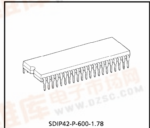
SDIP42-P-600-1.78 Weight : 4.13g (Typ.)
