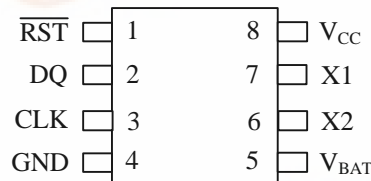
DS1602 8-Pin DIP (300-mil)
