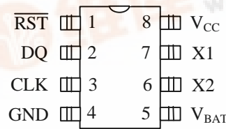
DS1602 8-Pin SOIC (200-mil)
