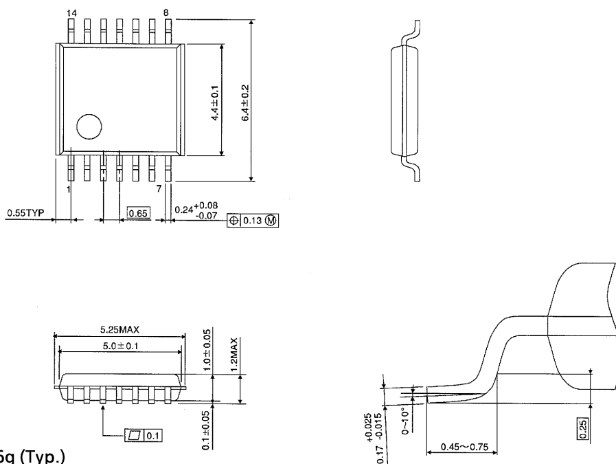
TSSOP 14PIN (170mil BODY) OUTLINE DRAWING (TSSOP14-P-0044-0.65)
