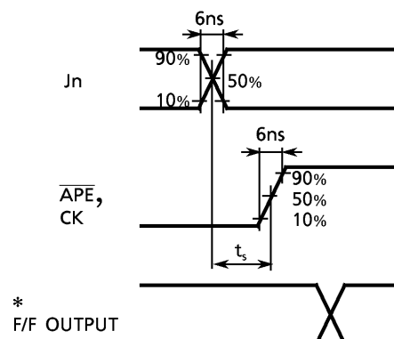
WAVEFORM 6
