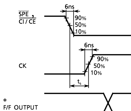
WAVEFORM 5
