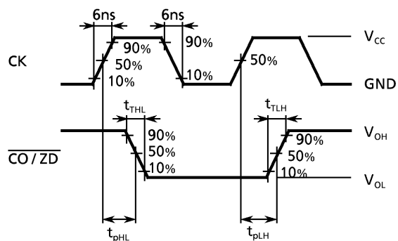
WAVEFORM 1
