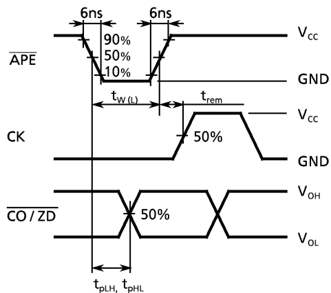
WAVEFORM 4
