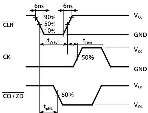
WAVEFORM 3
